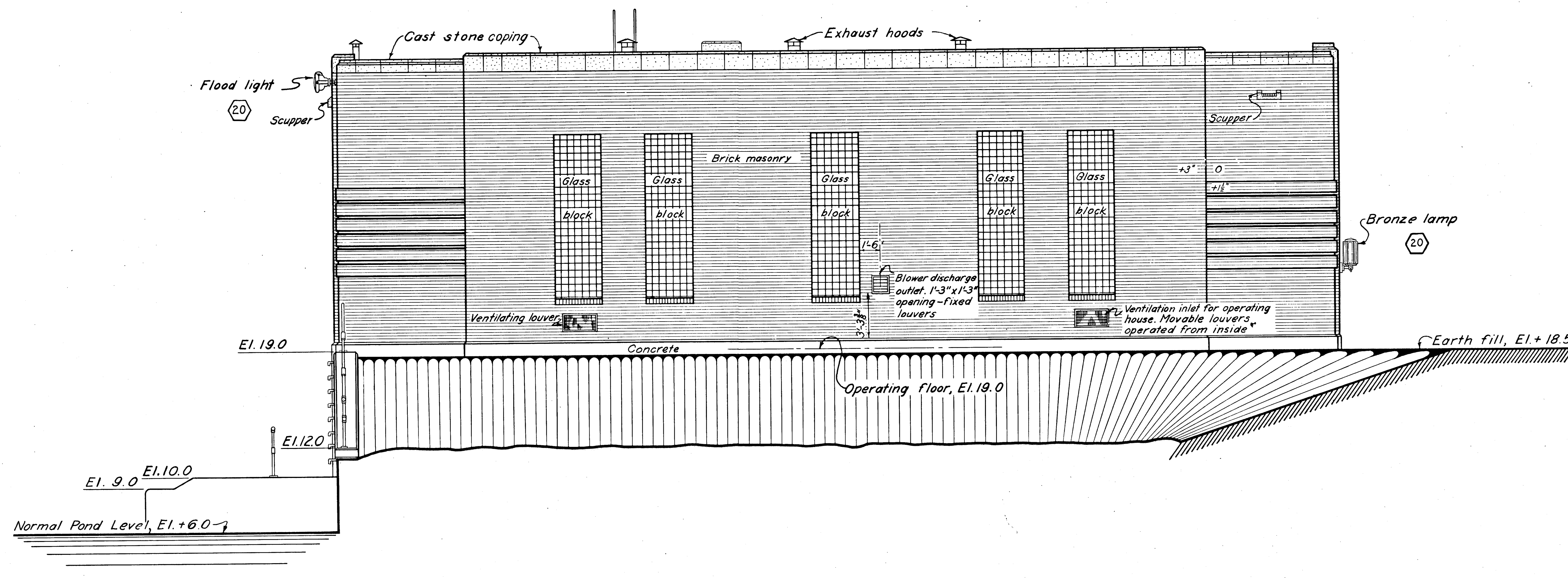
WEST ELEVATION SCALE \frac{1}{4}'' = 1'-0''
