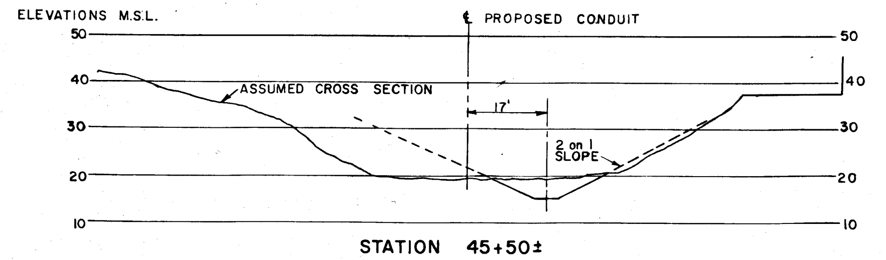
SECTIONS SECTIONS FACING UP-STREAM HOR. 1"=20' VERT. 1"=20'
