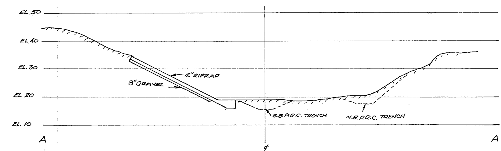
CROSS SECTION AT STATION 52+00 S.B.R.R.C. SCALE 1" = 20'-0"
