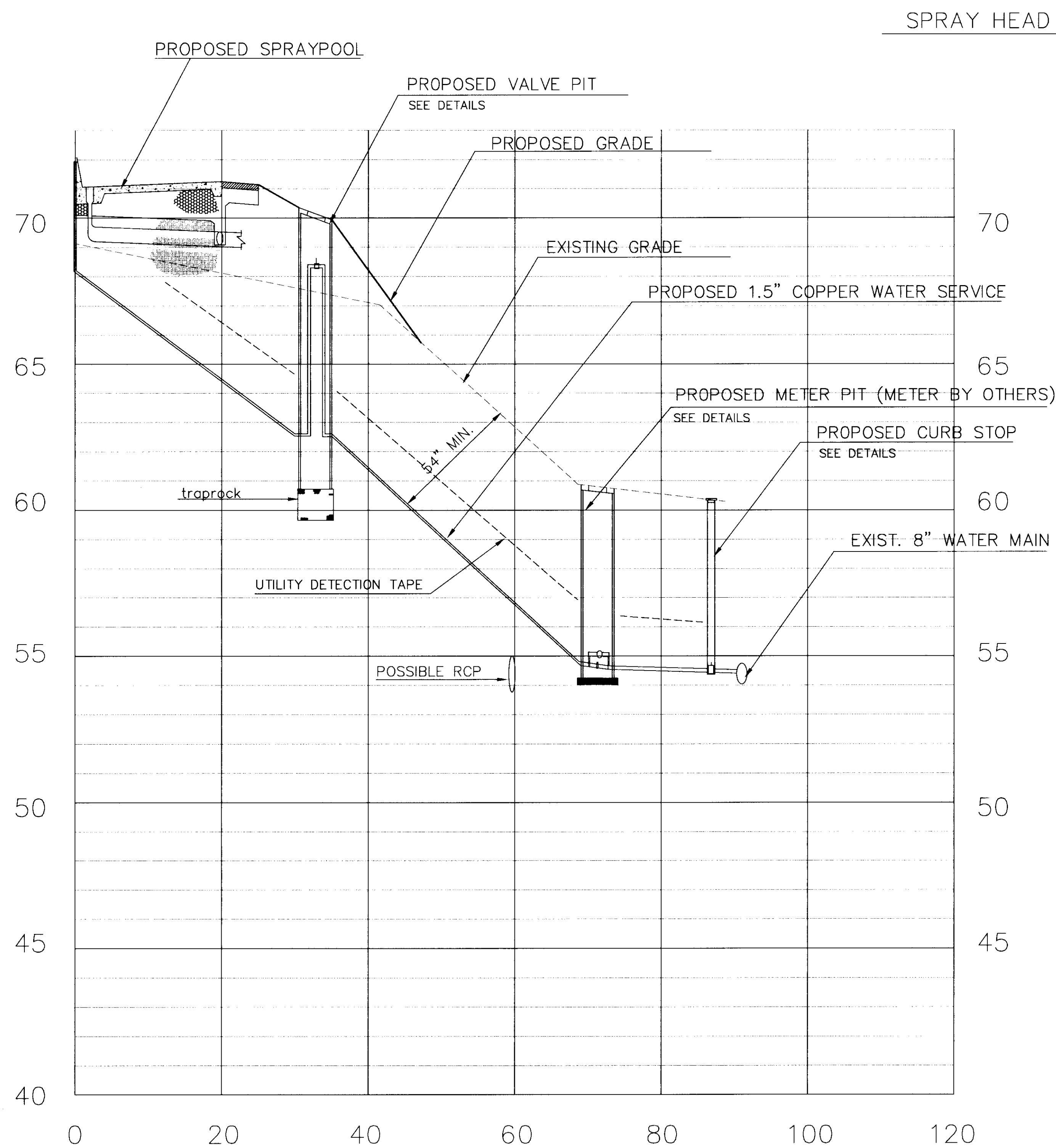
PROPOSED WATER CONNECTION
