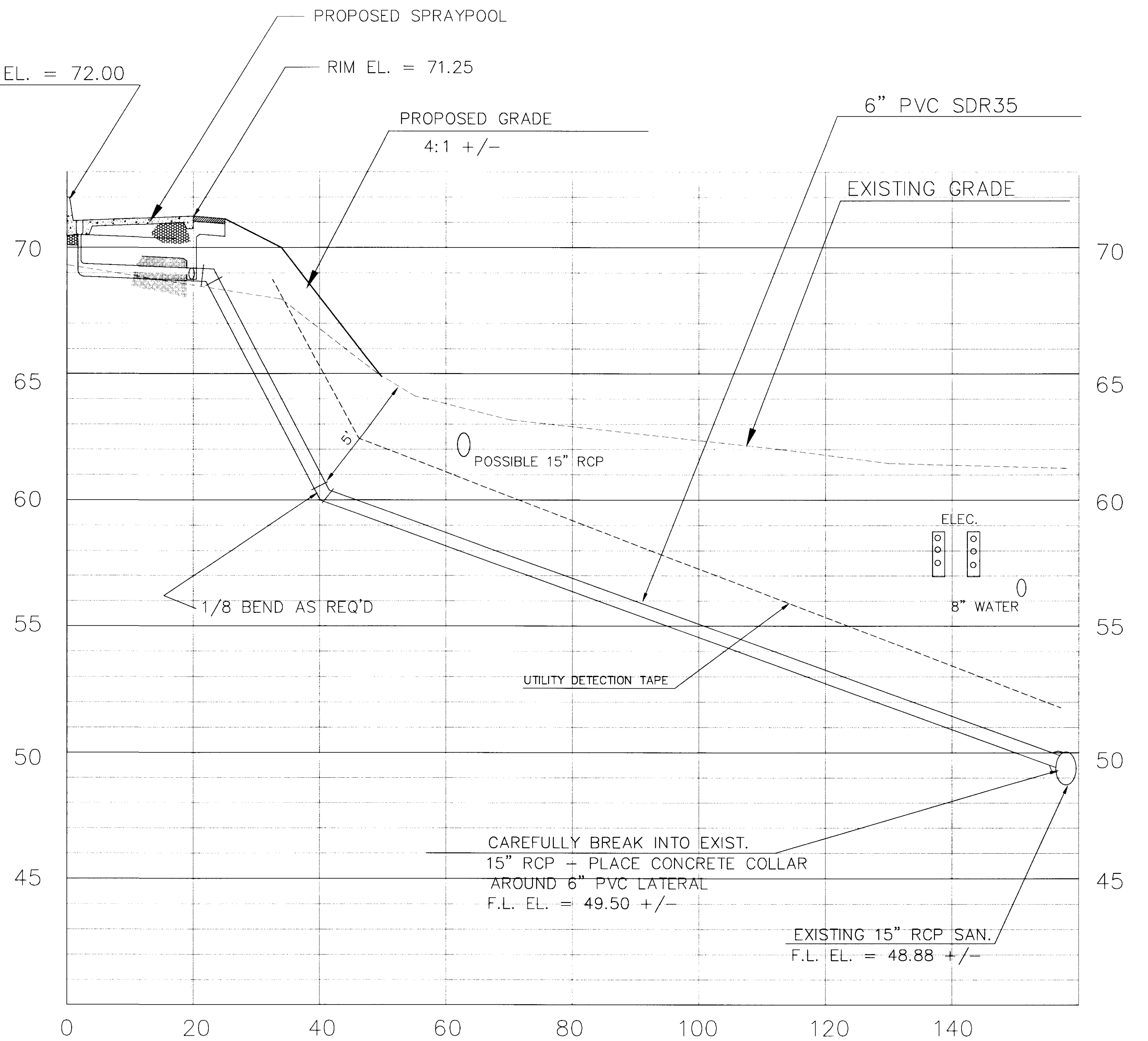
PROPOSED DIRECT LINE SANITARY CONNECTION
