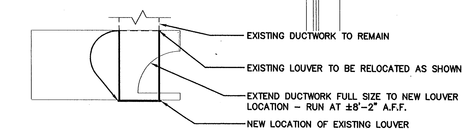
ELECTRIC ROOM PLAN - MECHANICAL
