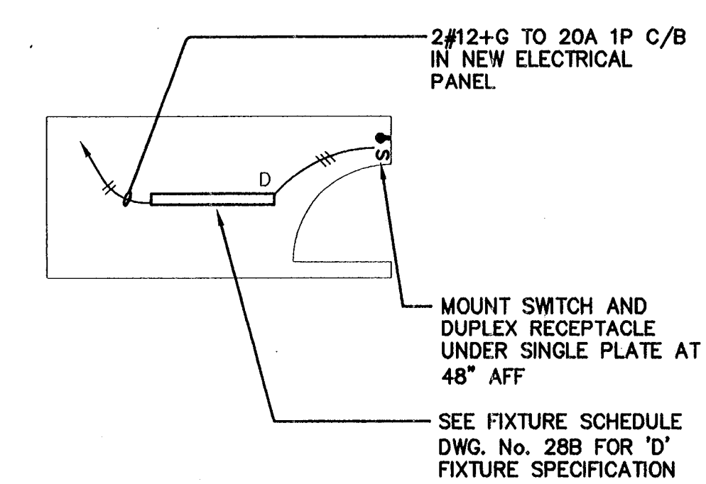
ELECTRIC ROOM PLAN - LIGHTING
