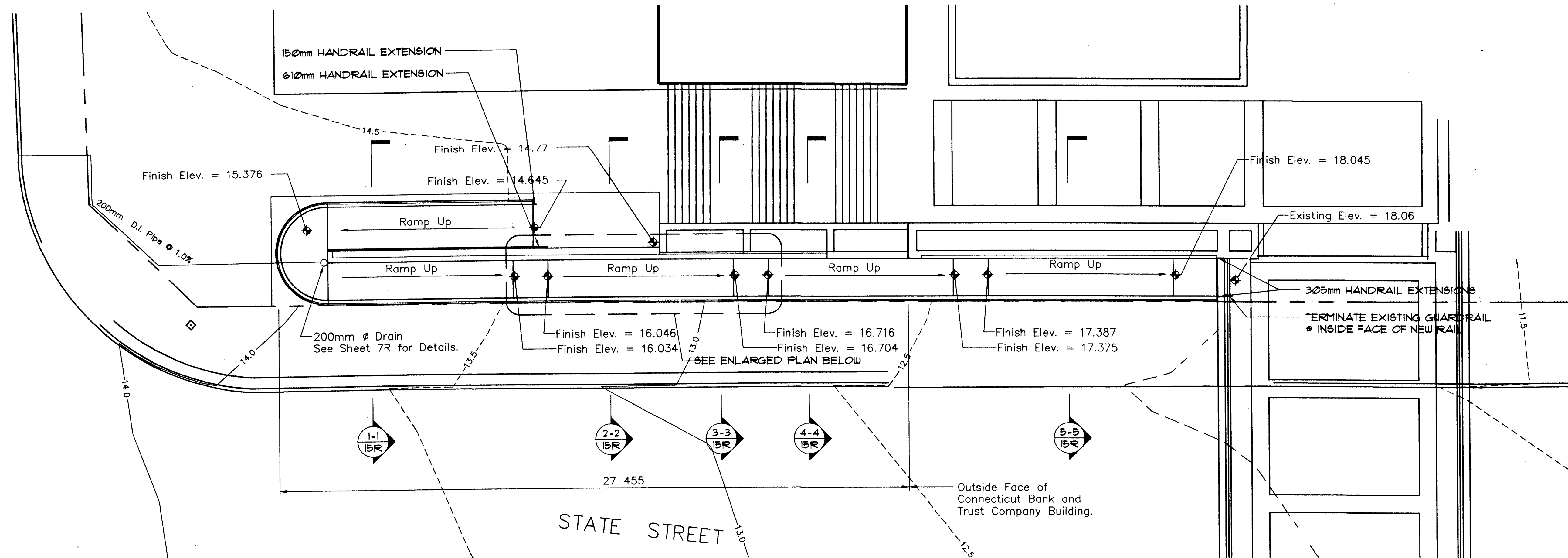
PRECAST AND GUARDRAIL PLAN SCALE 1:100
