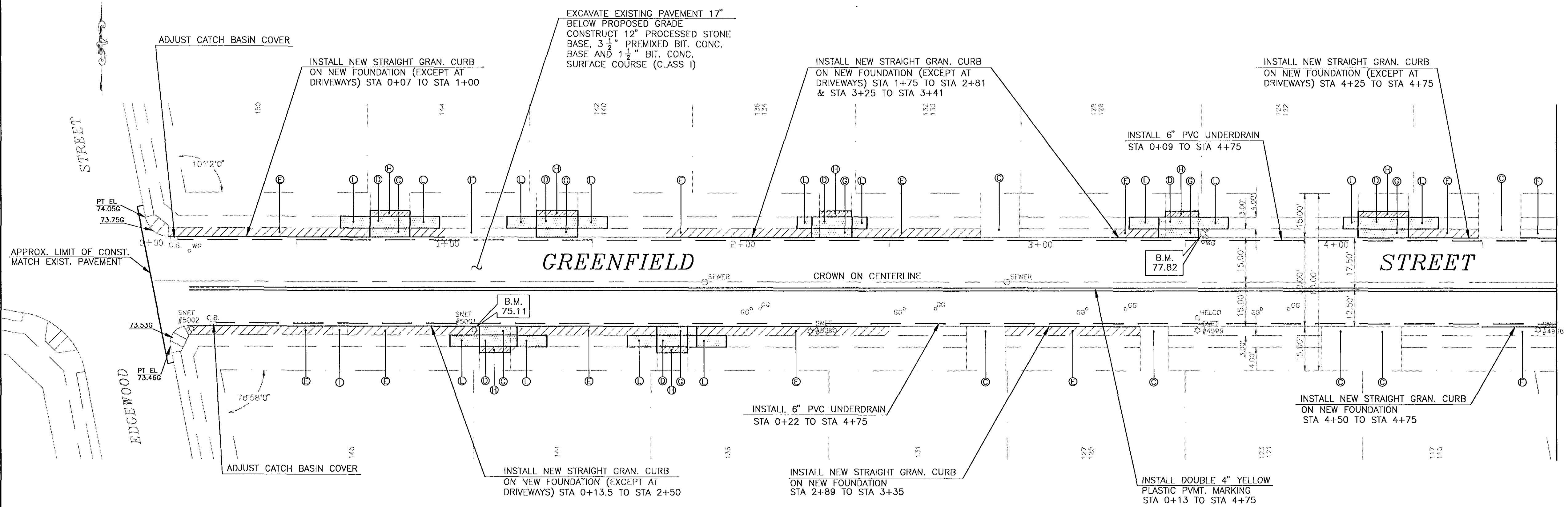
PLAN 1" = 20'
