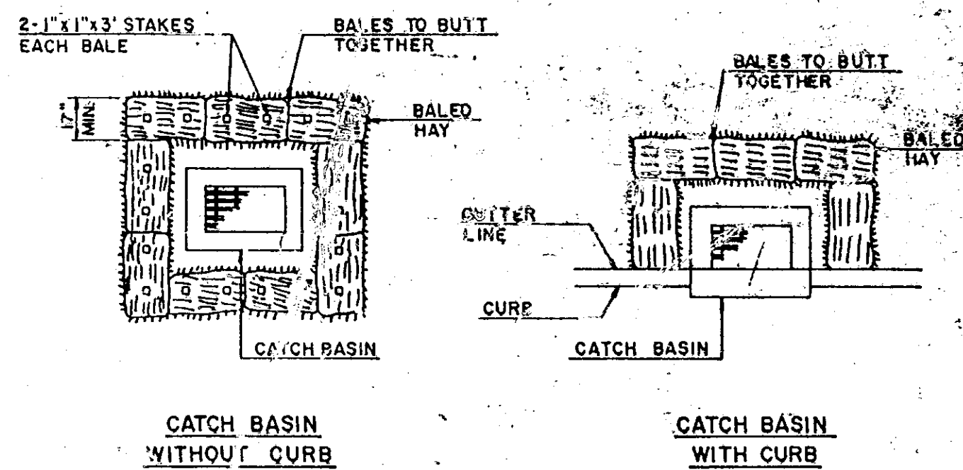
SEDIMENTATION CONTROL BALES
