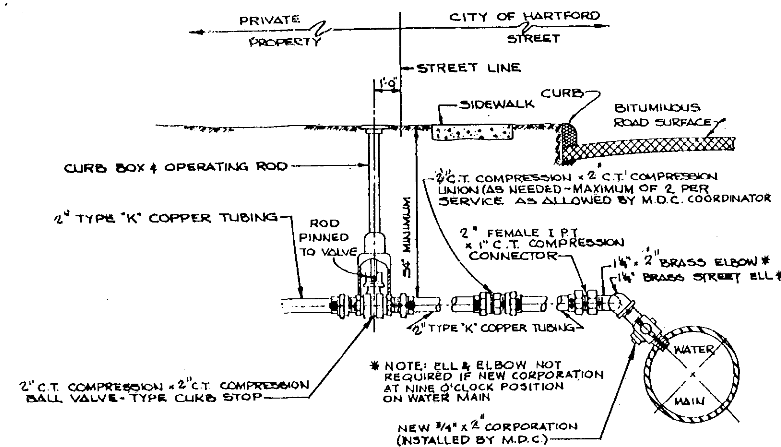
THE METROPOLITAN DISTRICT WATER SERVICE TYPICAL INSTALLATION DETAIL NTS
