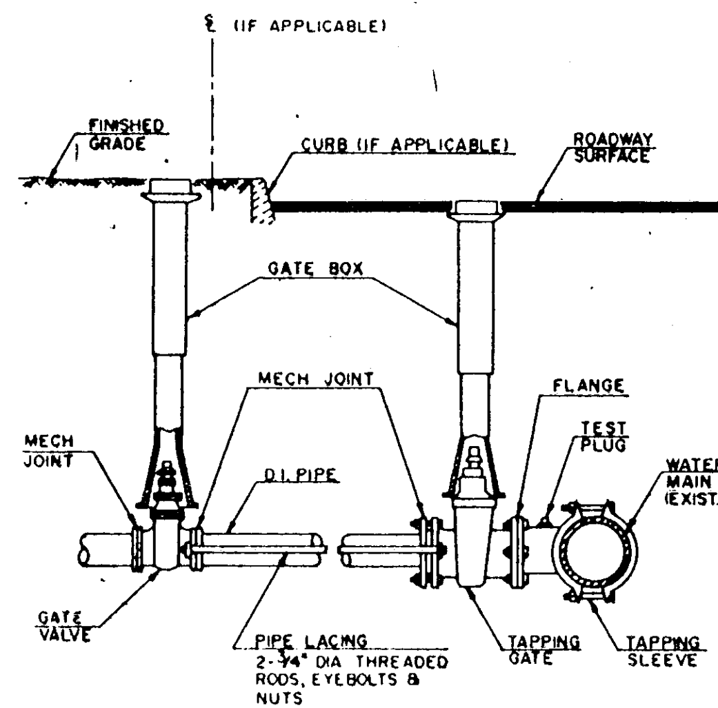
WATER SERVICES 4" THROUGH 8"
