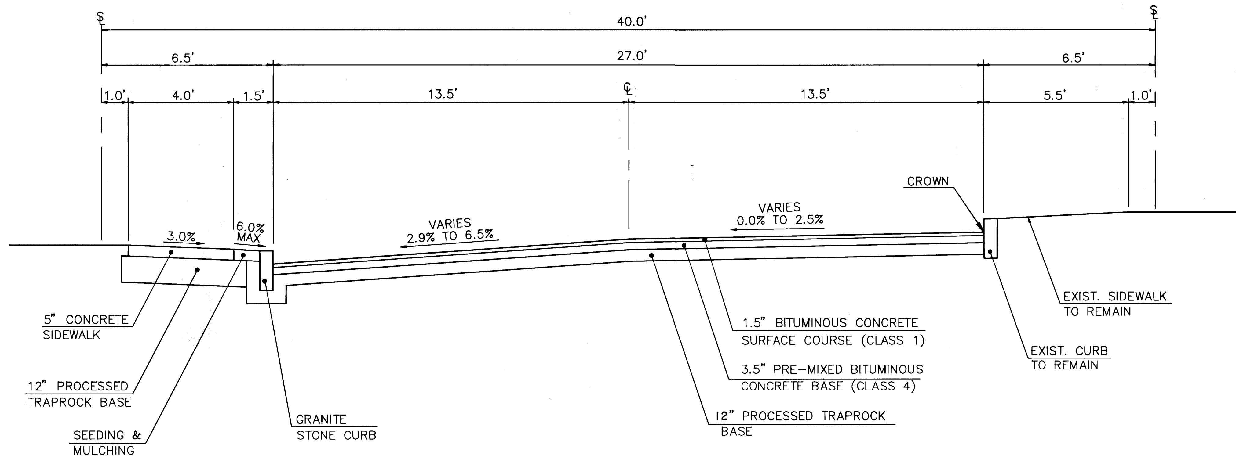
TYPICAL CROSS SECTION (TYPE 1)
