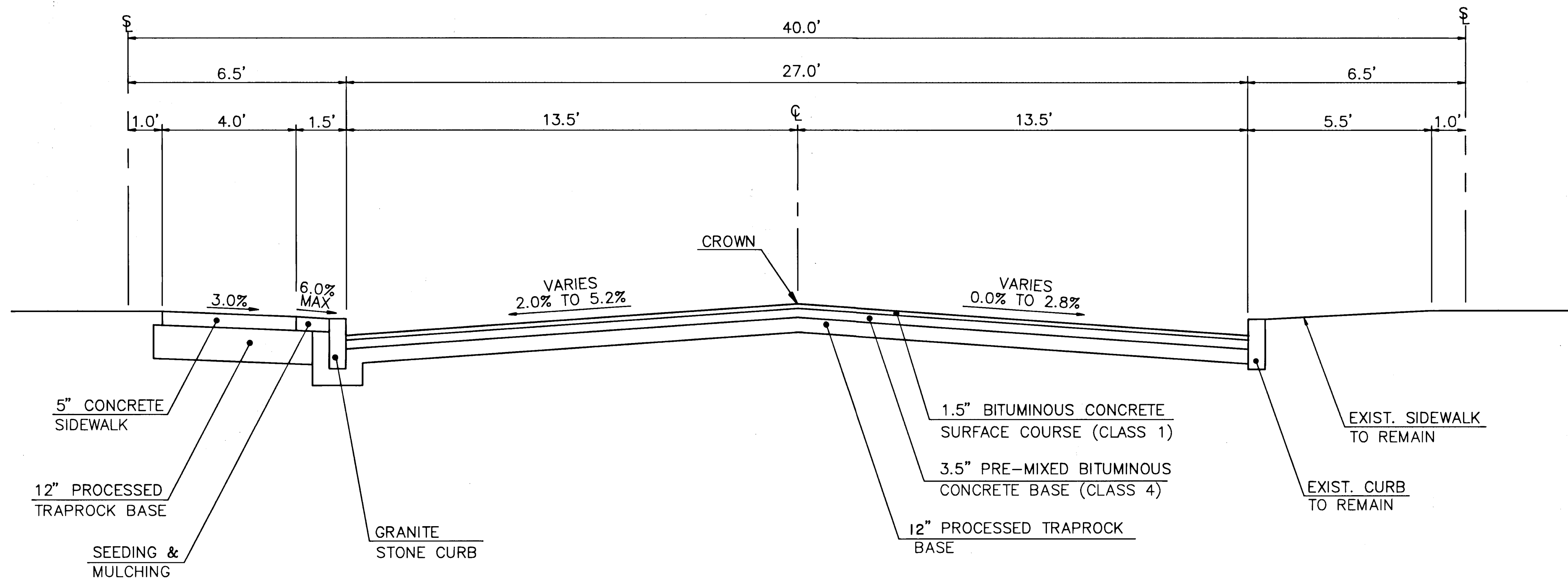
TYPICAL CROSS SECTION (TYPE 2)
