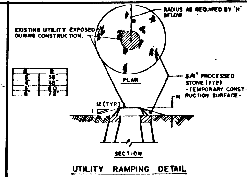
UTILITY RAMPING DETAIL
