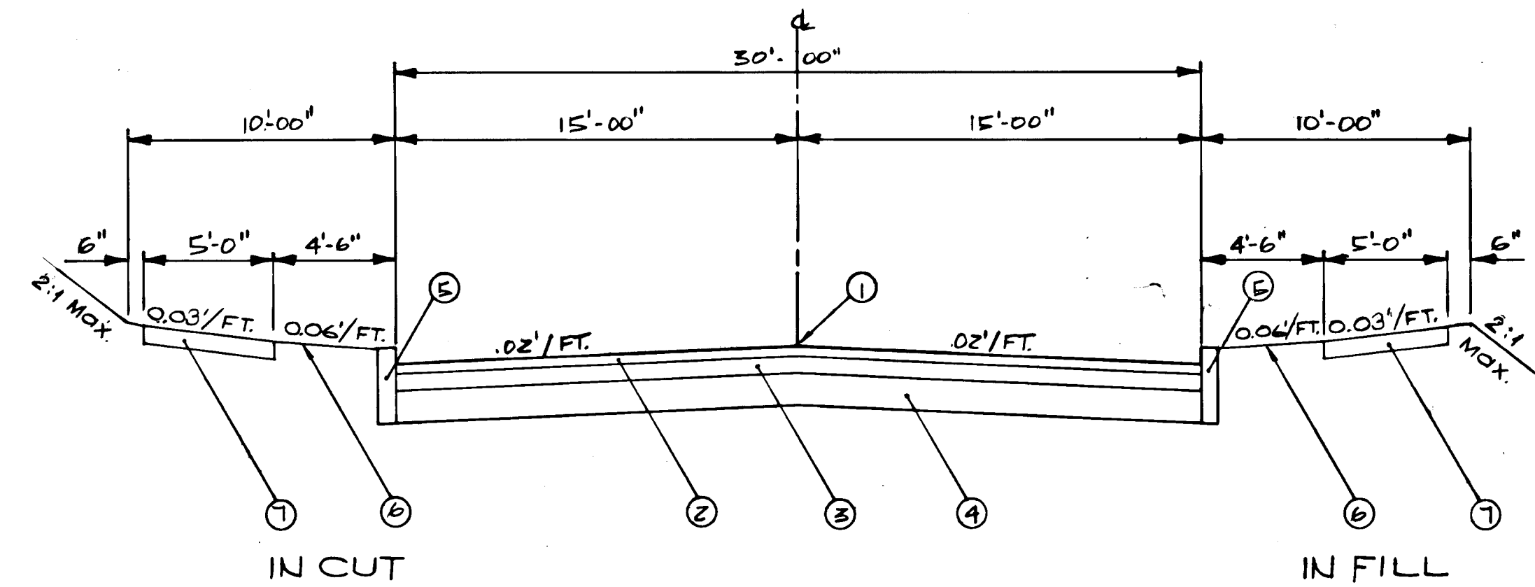
HOMESTEADING CUL-DE-SAC TYPICAL CROSS SECTION
