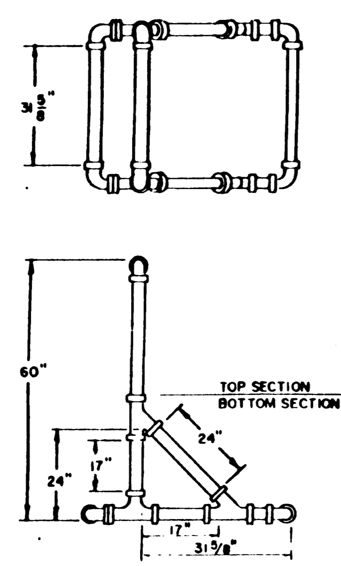
TYPICAL 3" OR 4" BARRICADE SUPPORT
