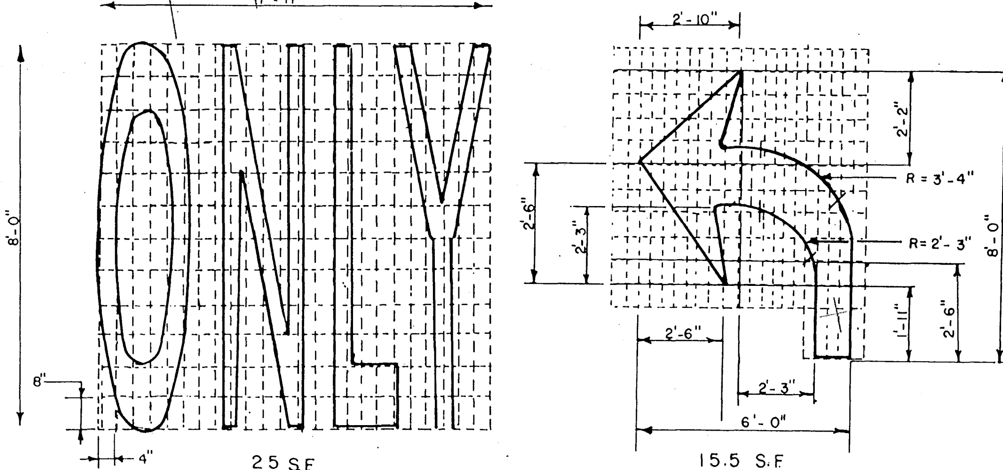
PAVEMENT MARKING DETAILS N.T.S.
