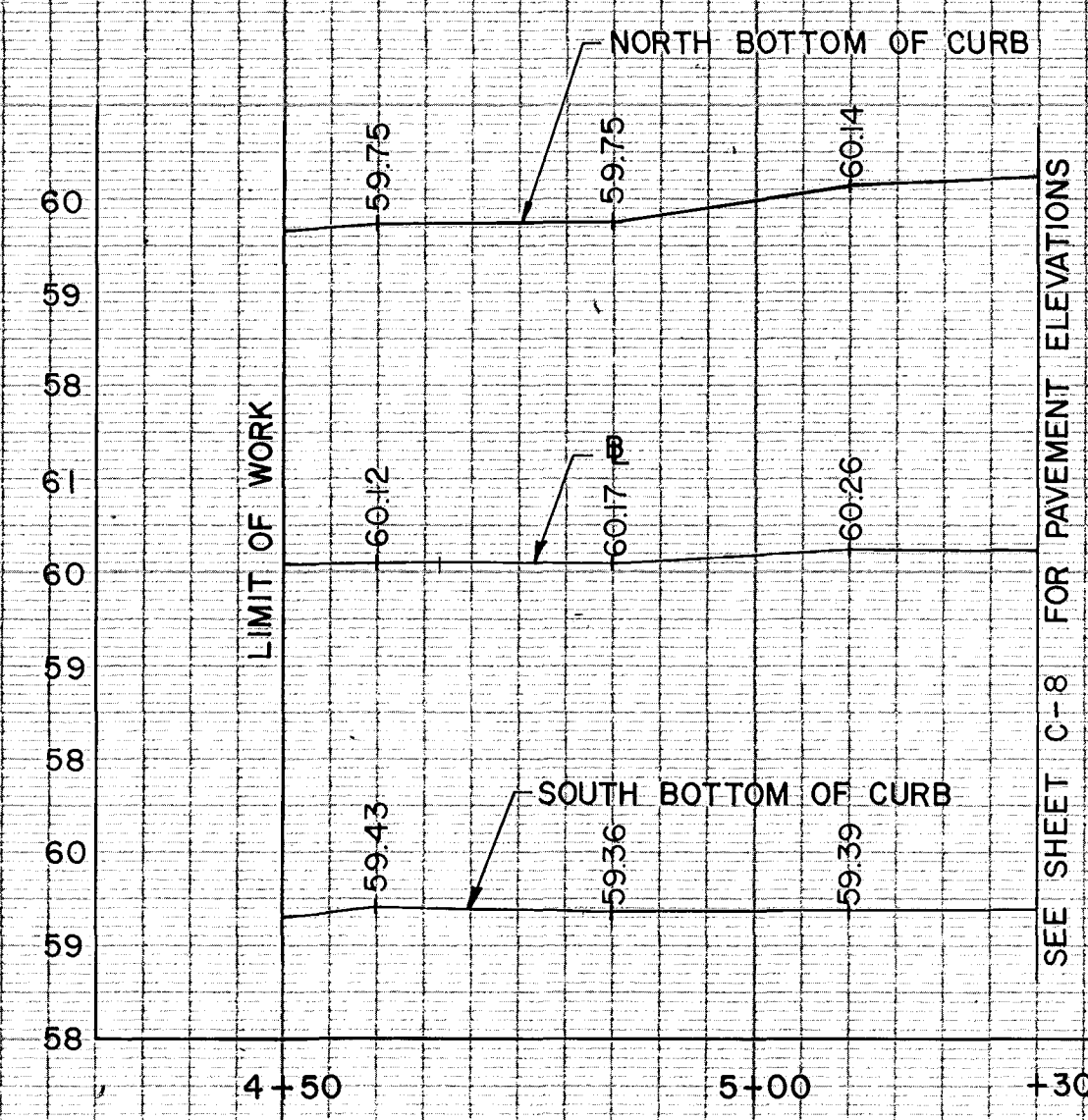
PEARL STREET PROFILE
