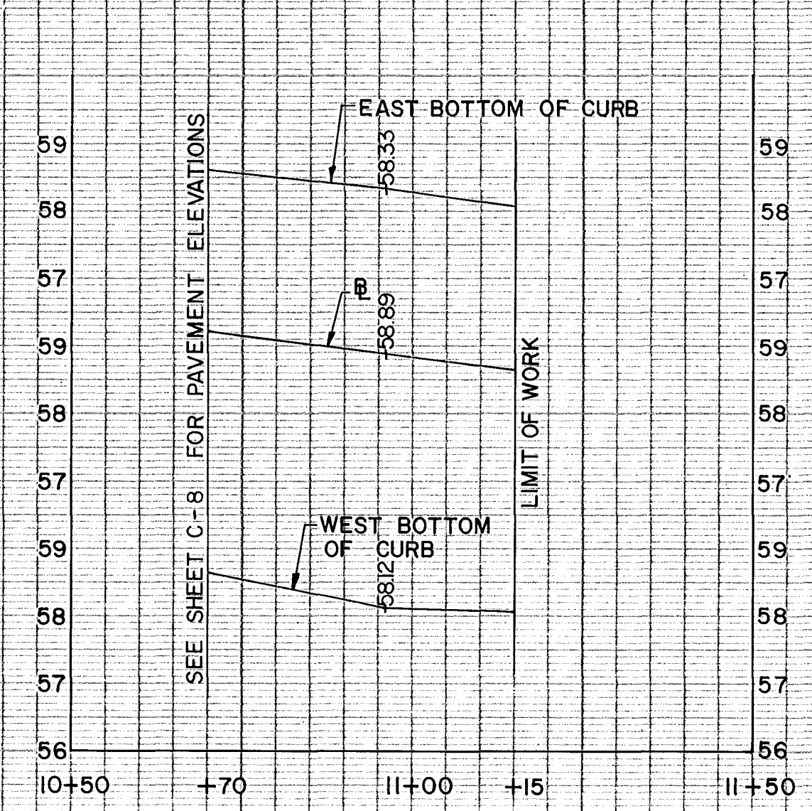
MAIN STREET PROFILE
