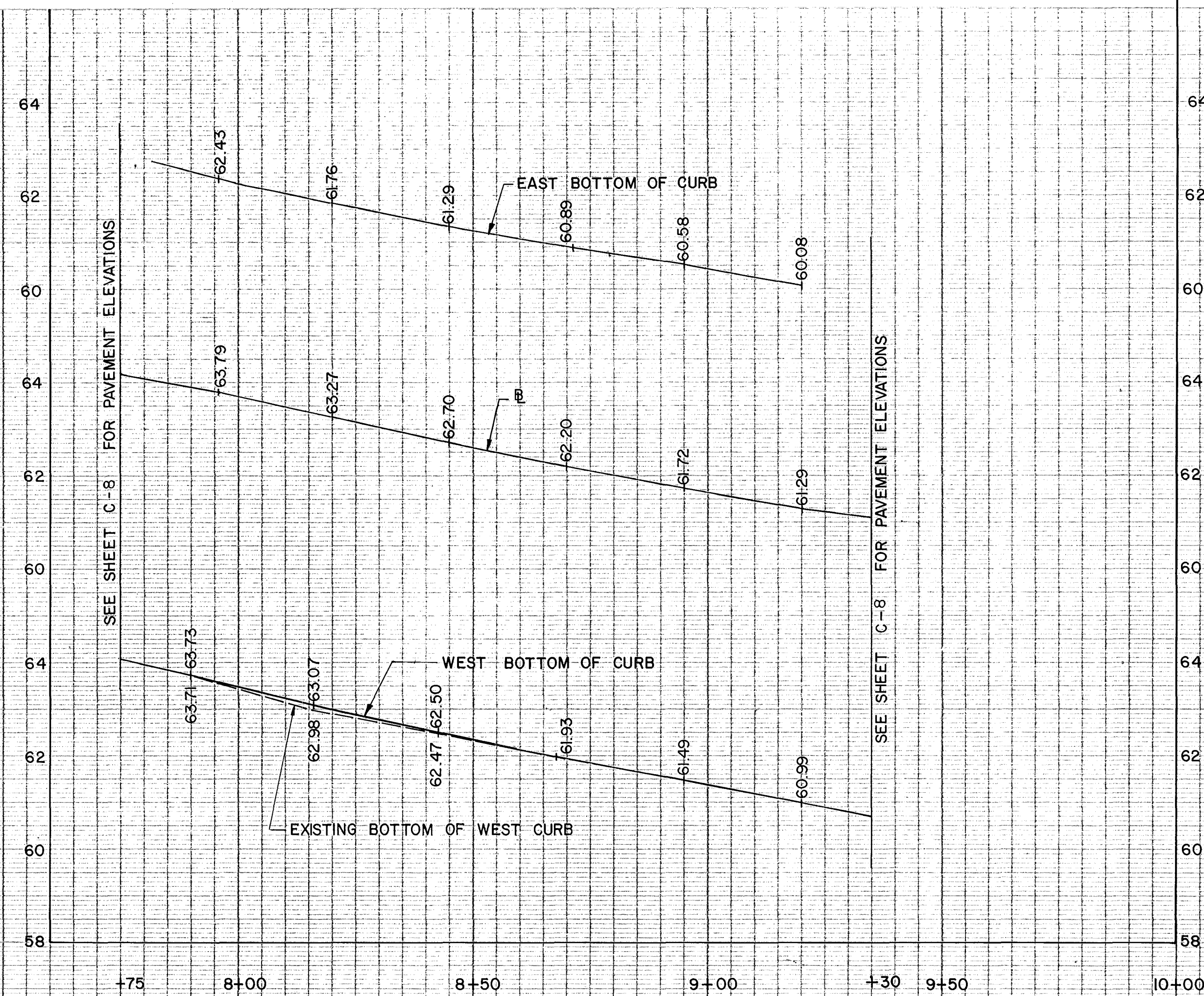
MAIN STREET PROFILE
