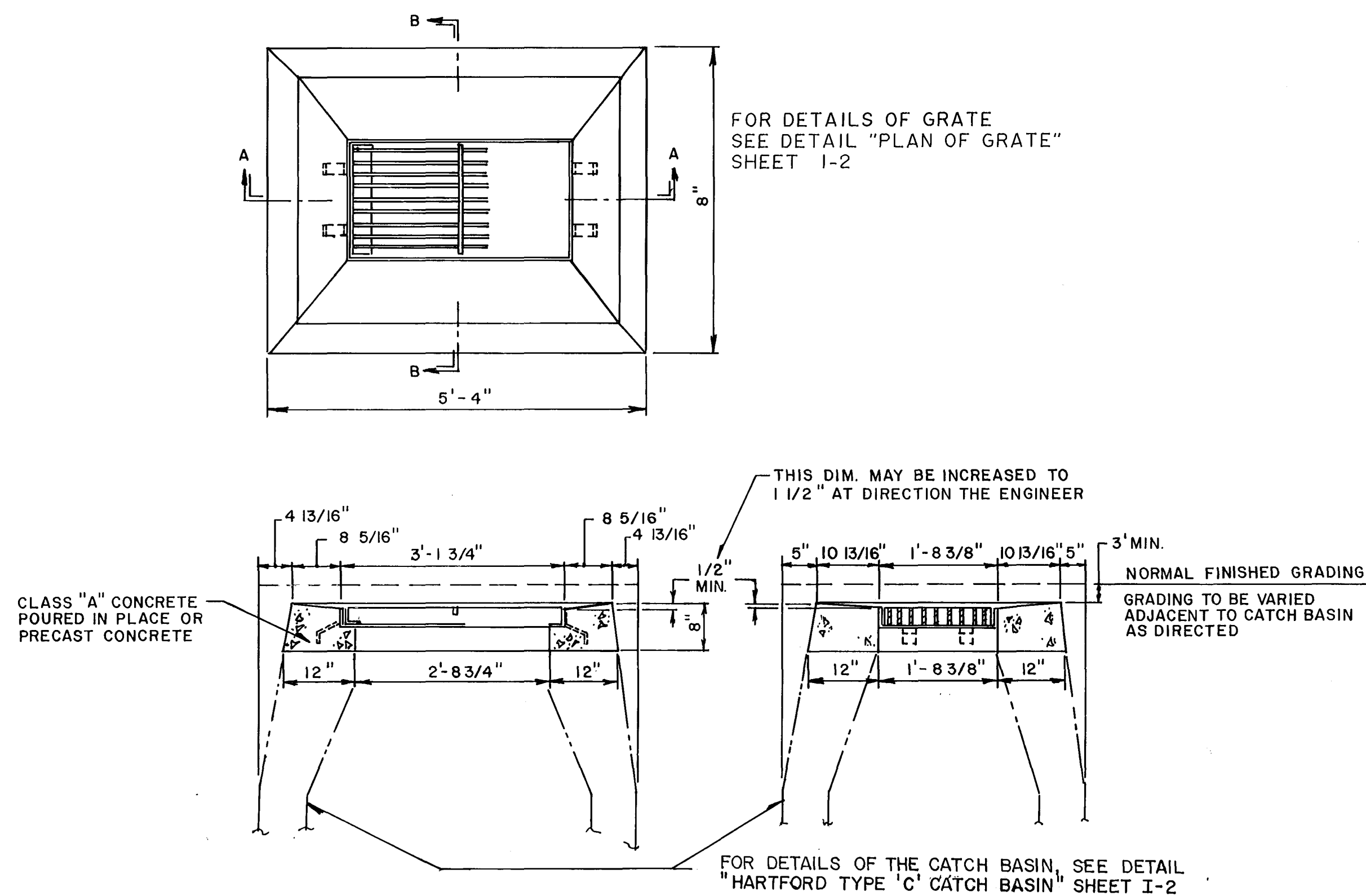
HARTFORD TYPE 'C-L' CATCH BASIN INLET
