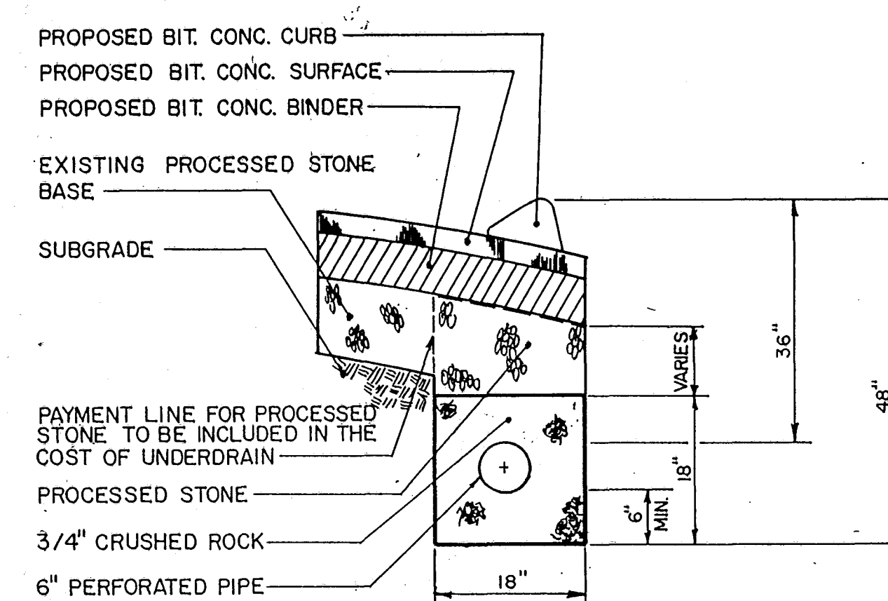
CURB UNDERDRAIN PAVEMENT REPAIR (DETAIL 2)
