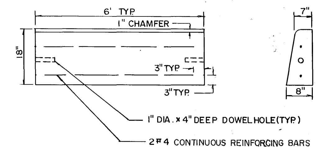
TYPICAL PRECAST CONCRETE CURB DETAIL
