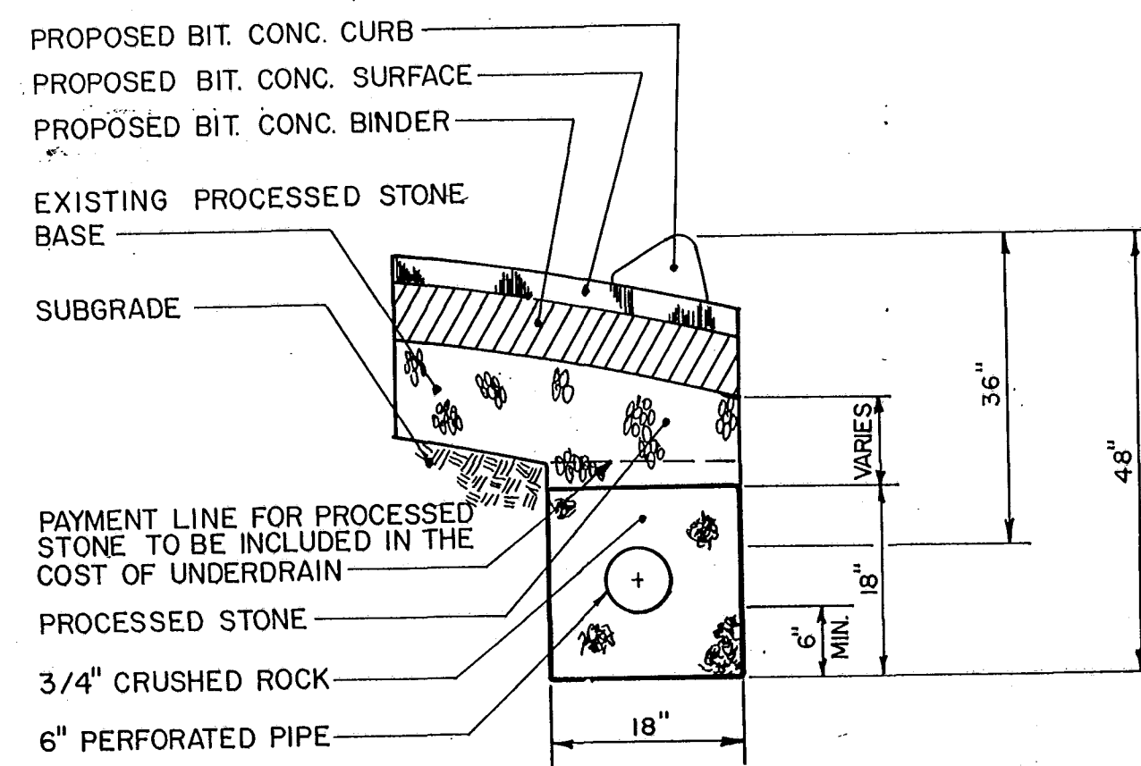
CURB UNDERDRAIN- TOTAL RECONSTRUCTION (DETAIL 1)
