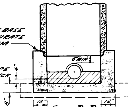
SECT. B-B
