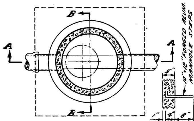
STEP DETAIL SCALE: 1"=2'-0"
