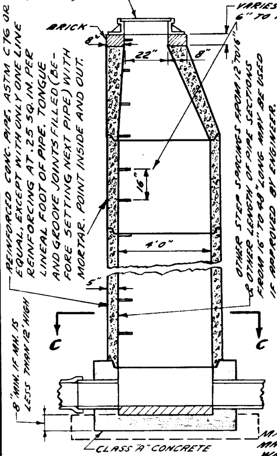
SECT. A-A
