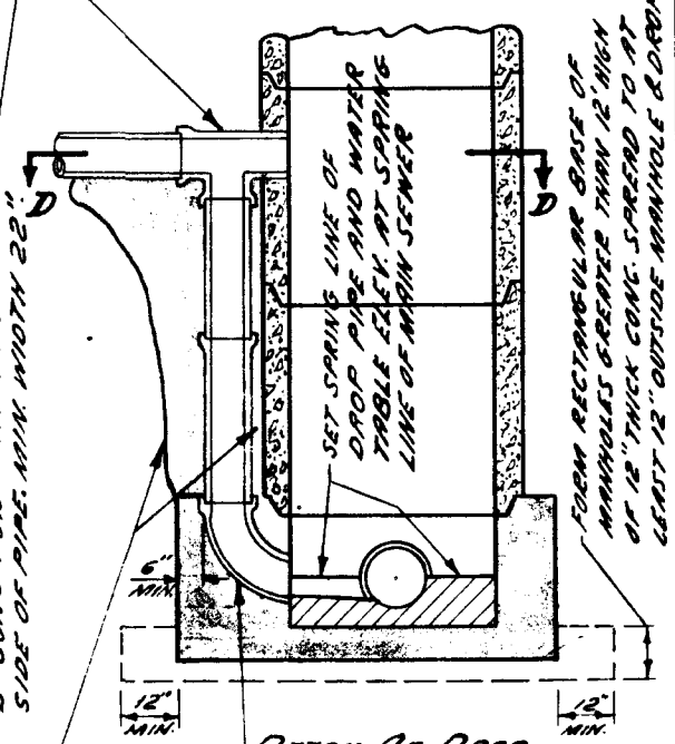
DETAIL OF DROP MANHOLE
