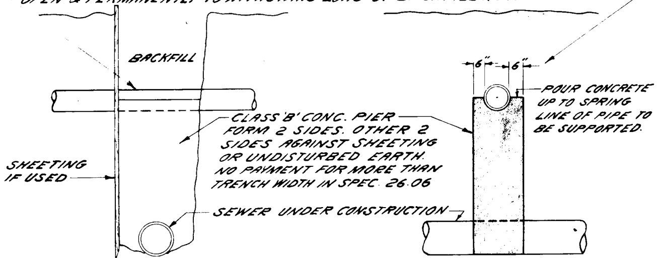
ELEVATION CROSS SECTION CONCRETE PIER AT SEWERS AND DRAINS
