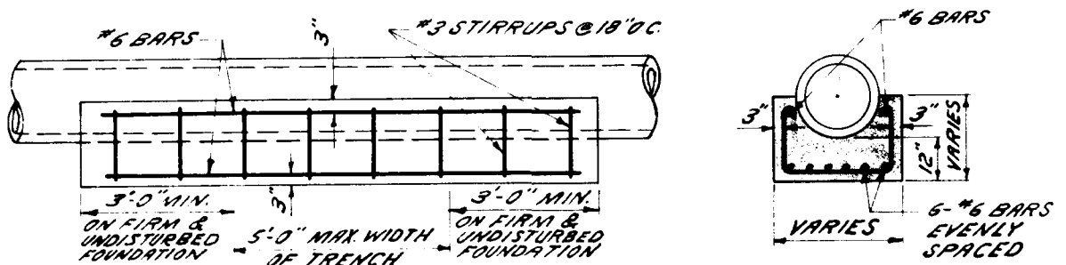
TYPICAL REINFORCED CONCRETE BEAM TO SUPPORT PIPES & DRAINS
