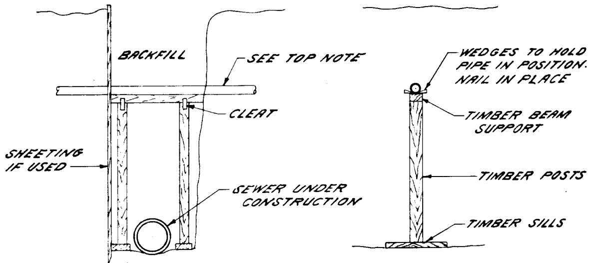
ELEVATION CROSS SECTION TIMBER PIPE SUPPORTS (TO BE AS DIRECTED BY UTILITY COMPANY CONCERNED)
