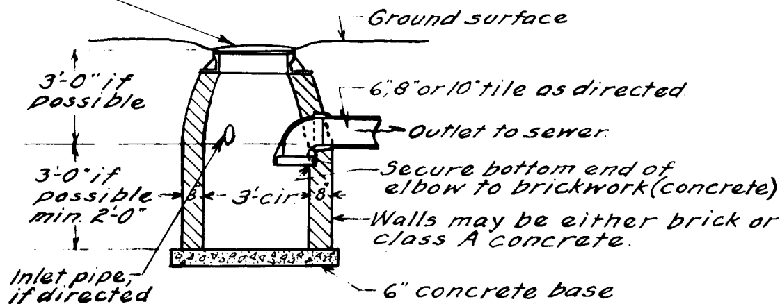
Permanent Catch-Basin or for use in large areas
