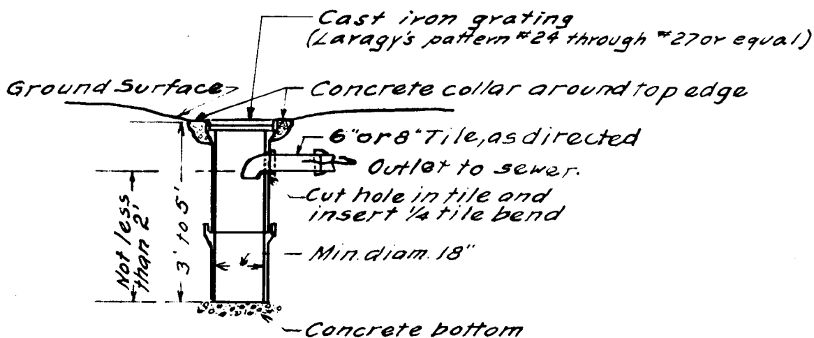
Catch-basin for single lot or small area.
