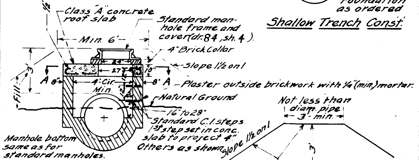
Sect. B-B
