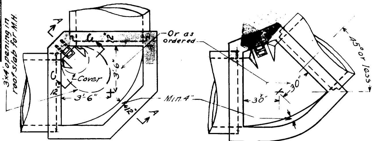
Sect. B-B
