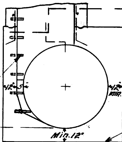
Sect. A-A
