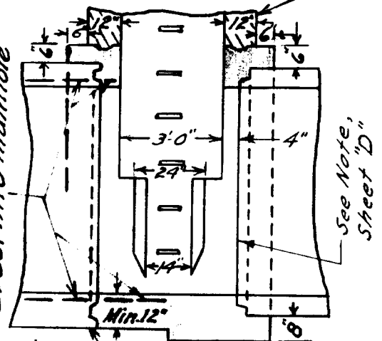
Sect. B-B
