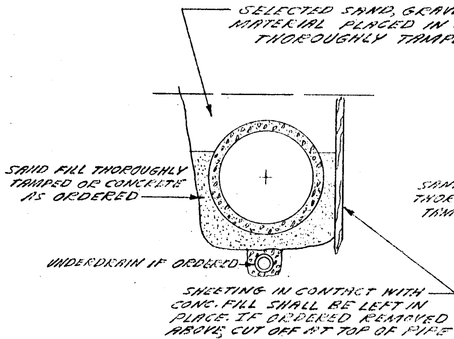
PIPE IN SOFT OR WET MATERIAL
