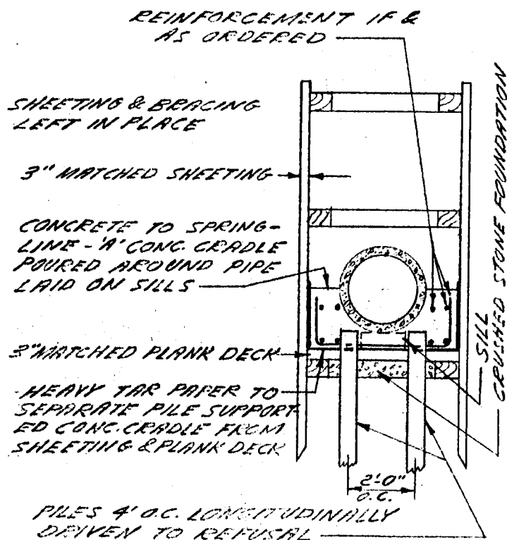
SPECIAL CONCRETE SEWER FOUNDATION WITH PILES
