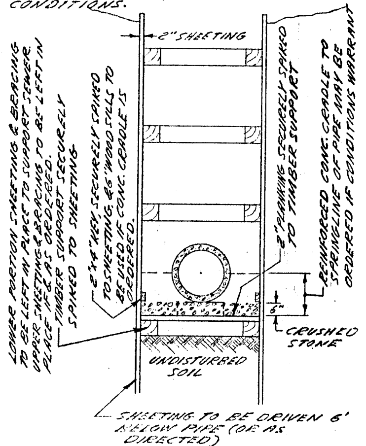
SPECIAL SEWER FOUNDATION FOR INADEQUATE SOIL CONDITIONS
