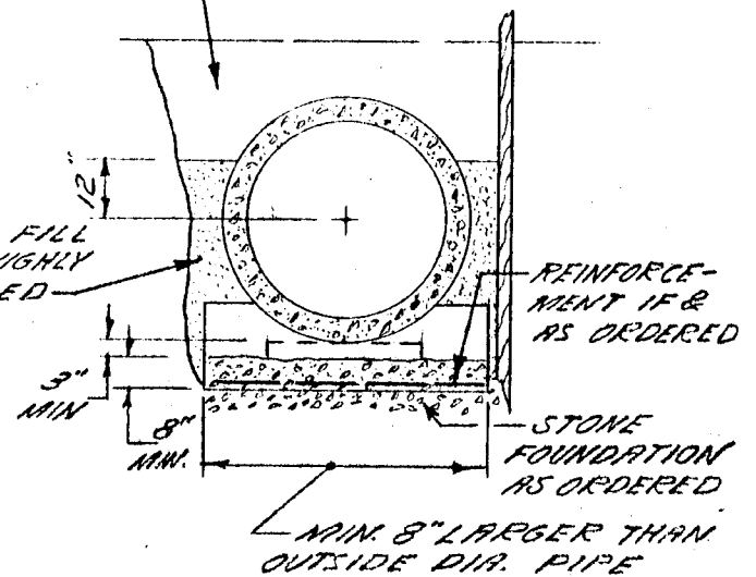
PIPE ON PRE-BUILT CRADLE
