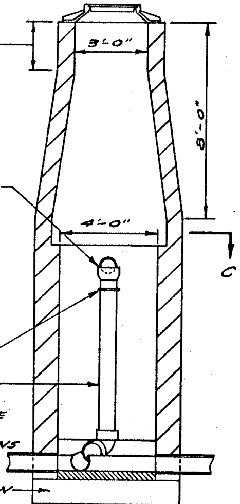
SECTION B-B
