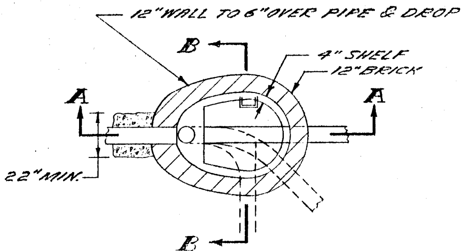
SECTION C-C
