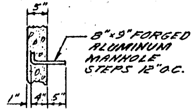
STEP DETAIL SCALE: 1"=2'-0"
