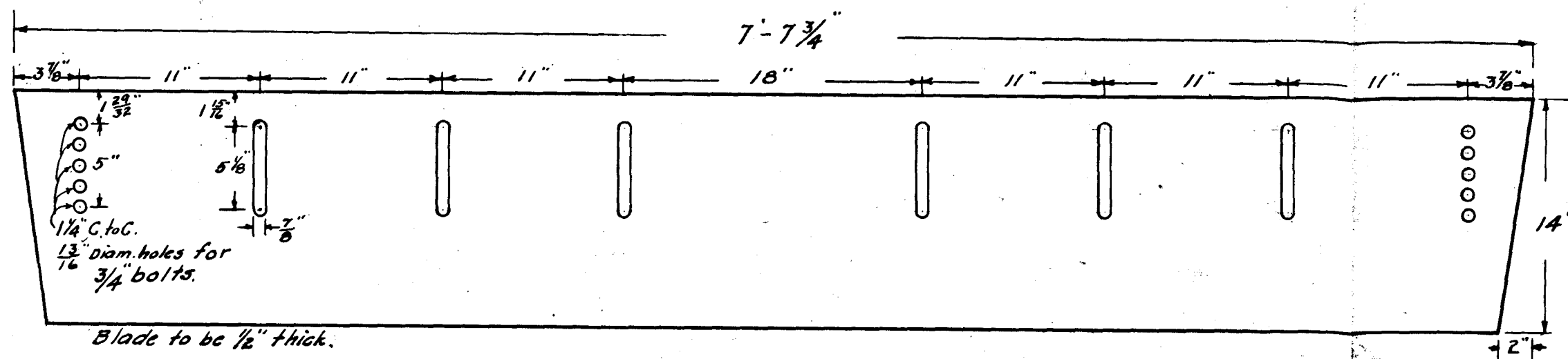
BLADE FOR SNOW LOADERS No. 45-46-47-48-54.
