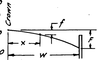
0.80 PAVEMENT SECTION
