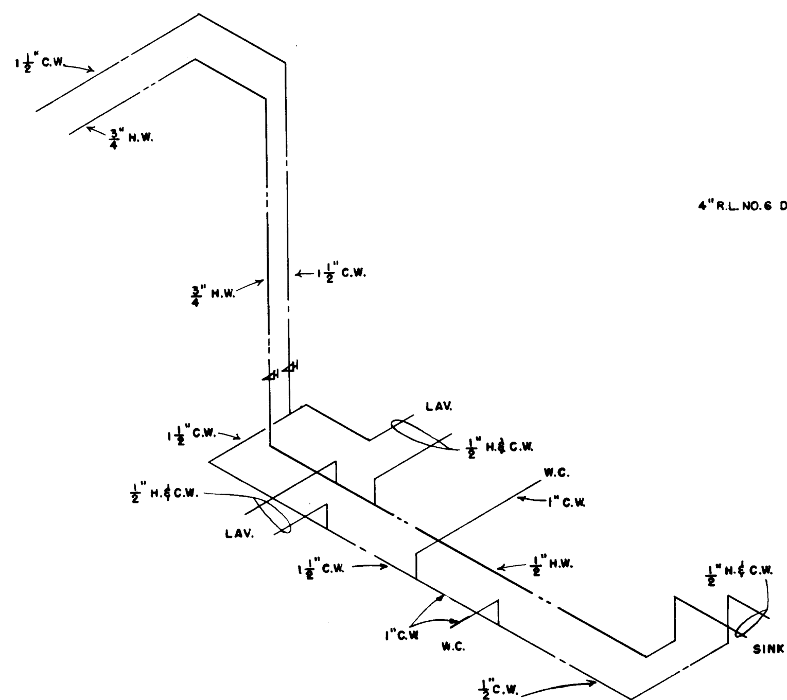
BOY'S & GIRL'S TOILETS - SECOND FLOOR WATER RISER DIAGRAM
