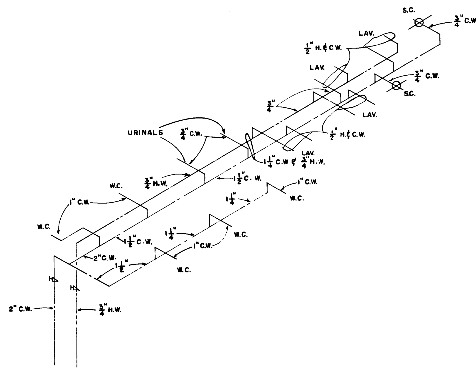
MEN'S & WOMEN'S TOILETS 2ND FLOOR WATER RISER DIAGRAM
