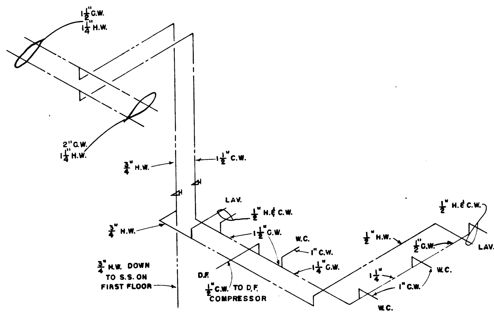
MEZZANINE TOILET ROOM WATER RISER DIAGRAM
