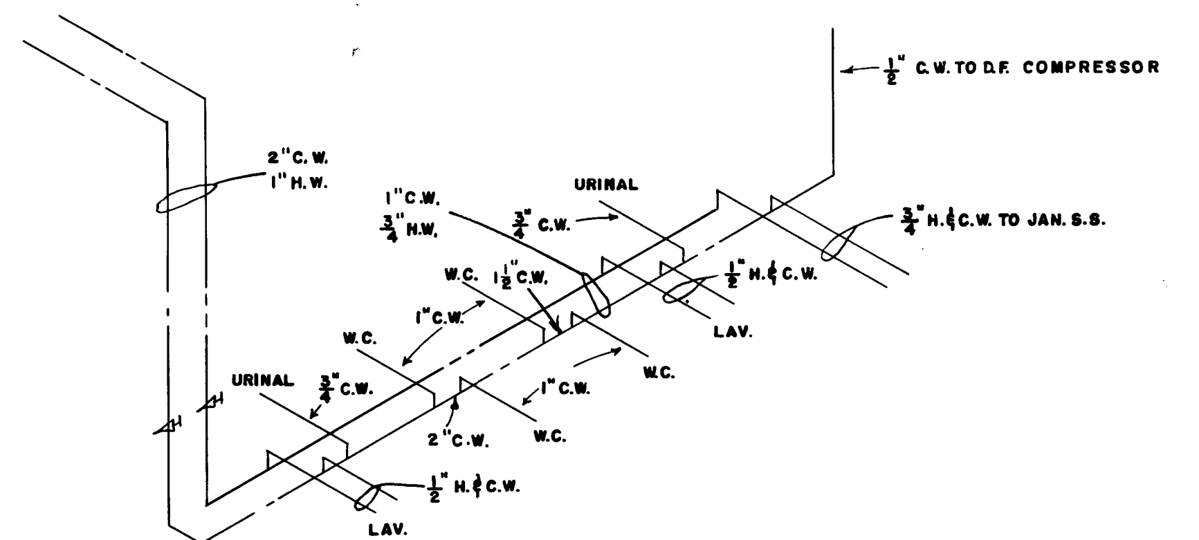
MEN'S & WOMEN'S TOILETS - BASEMENT WATER RISER DIAGRAM
