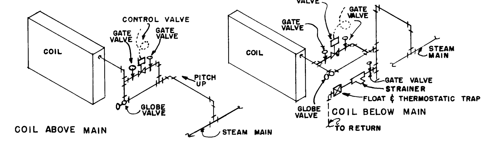
STEAM CONNECTIONS TO COILS NOT TO SCALE
