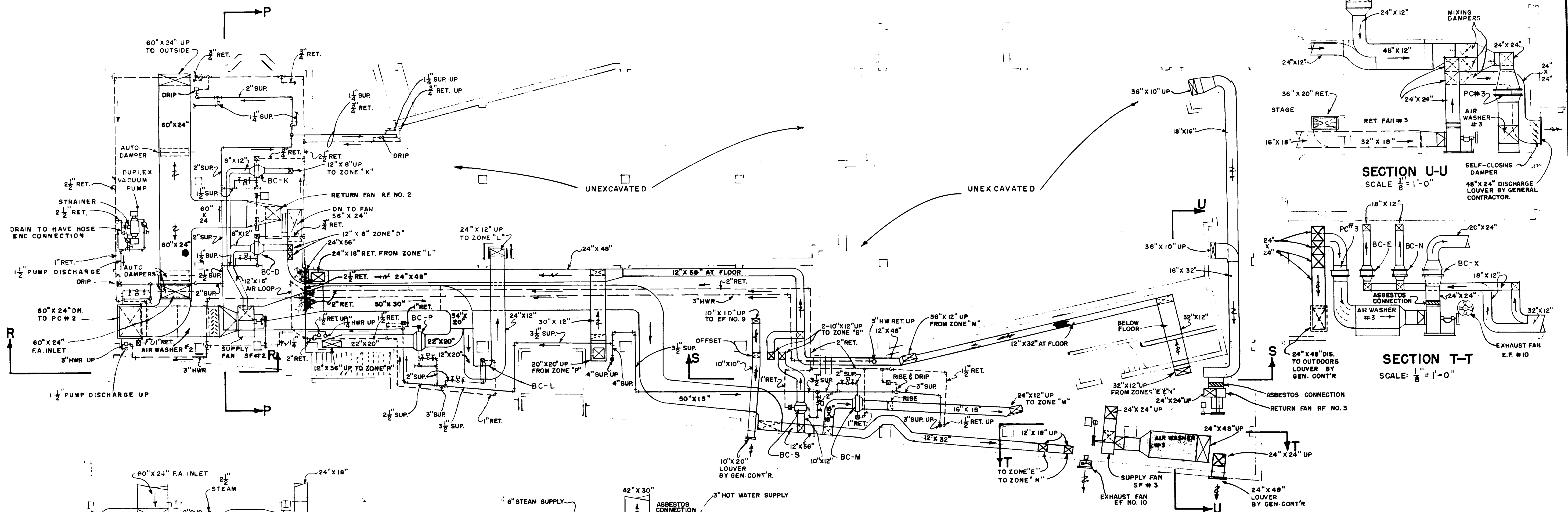
SUB-BASEMENT PLAN (SOUTH SIDE OF HIGHWAY) HEATING & VENTILATING SCALE: \frac{1}{8}'' = 1'-0''
