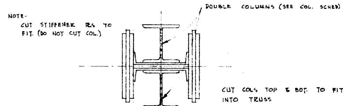
TYPICAL DETAIL OF DOUBLE COLUMN AT END MEMBER OF TRUSS SCALE: 1/4"=1'-0"
