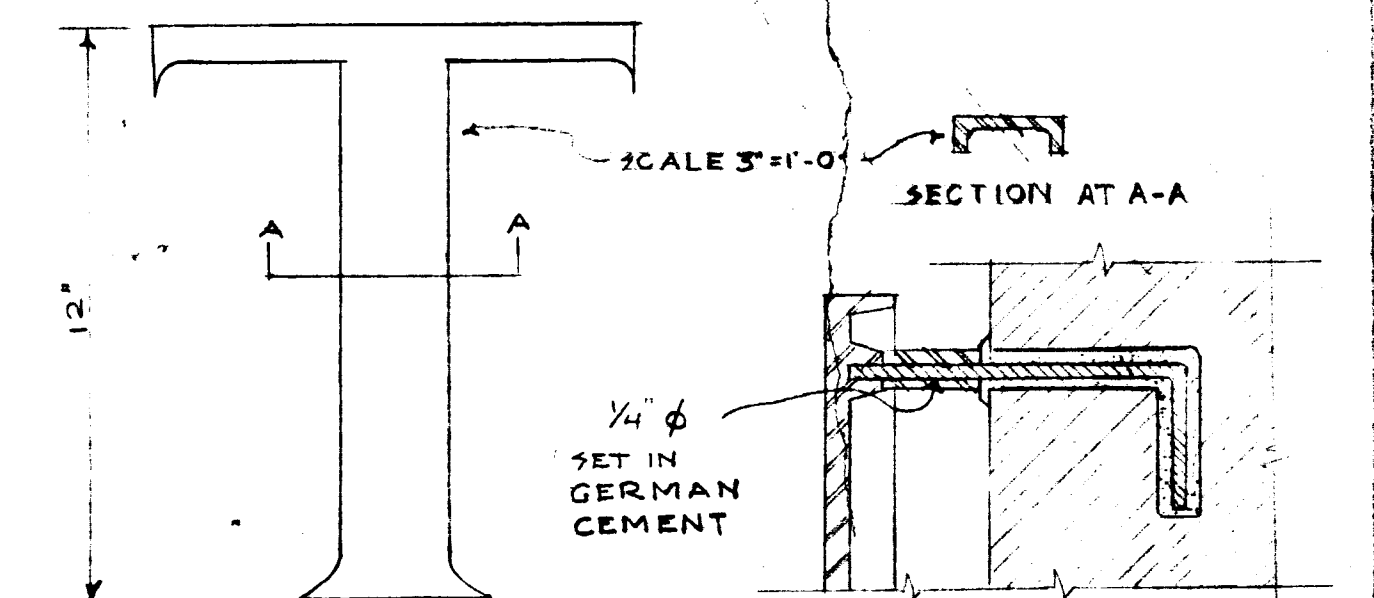
DETAIL OF FASTENING METAL LETTERS SCALE 1/2" = 1'-0"
