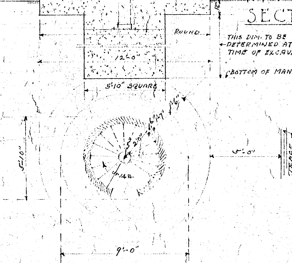
PLAN B-B
