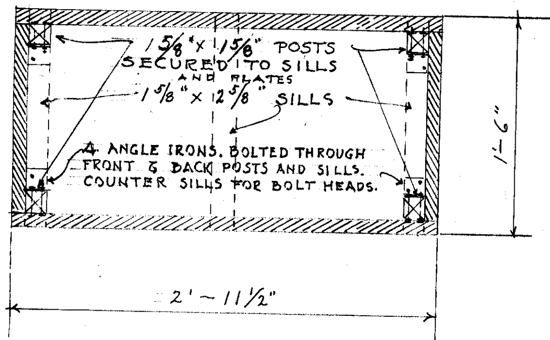
PLAN
