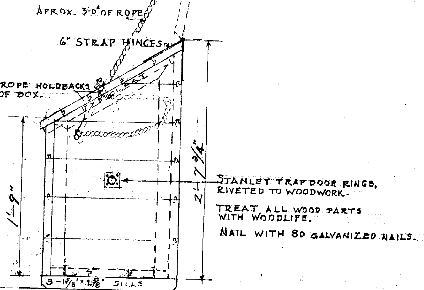
END VIEW
