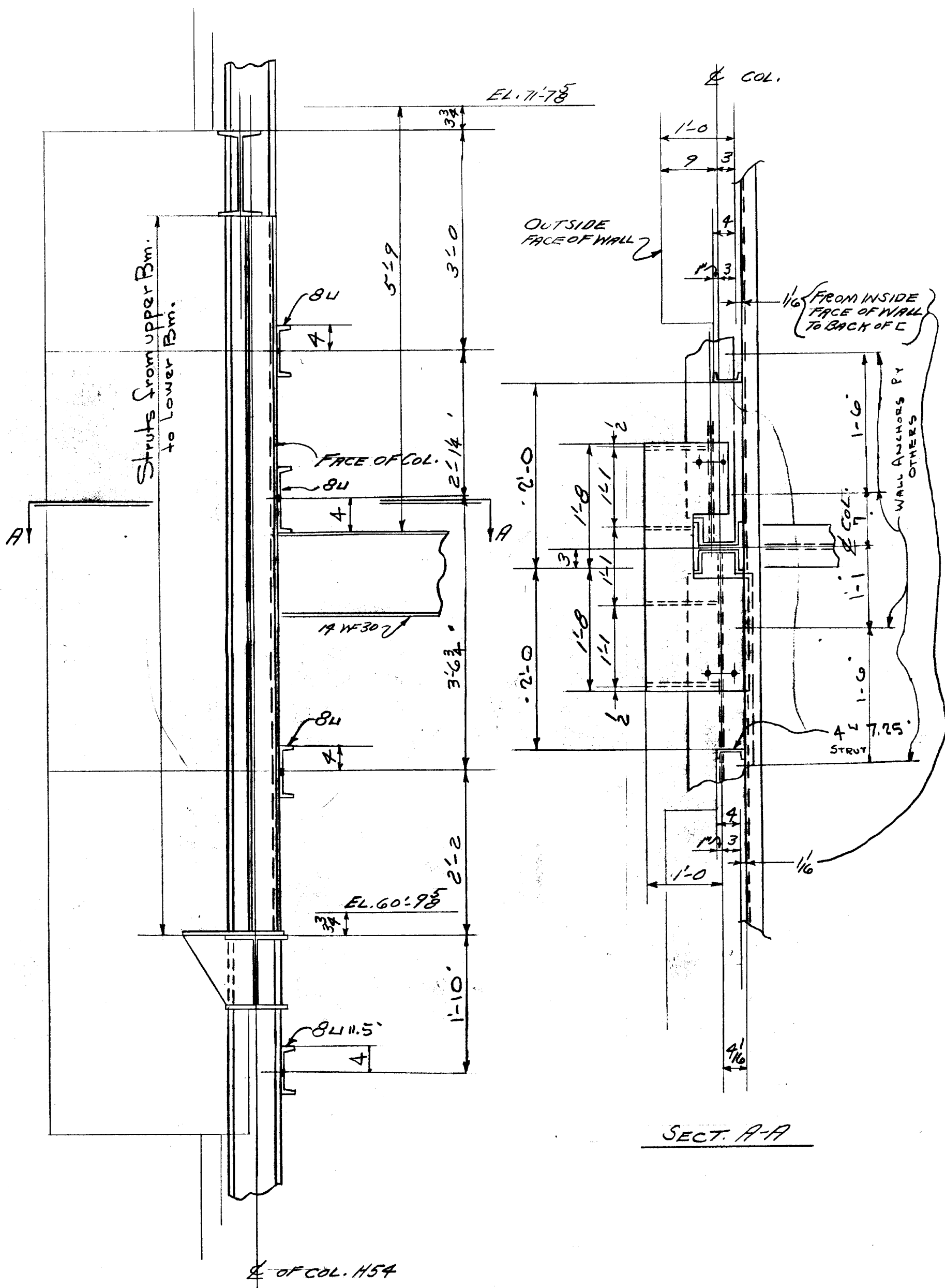
LAYOUT FOR MARBLE BLOCK SUPPORT
