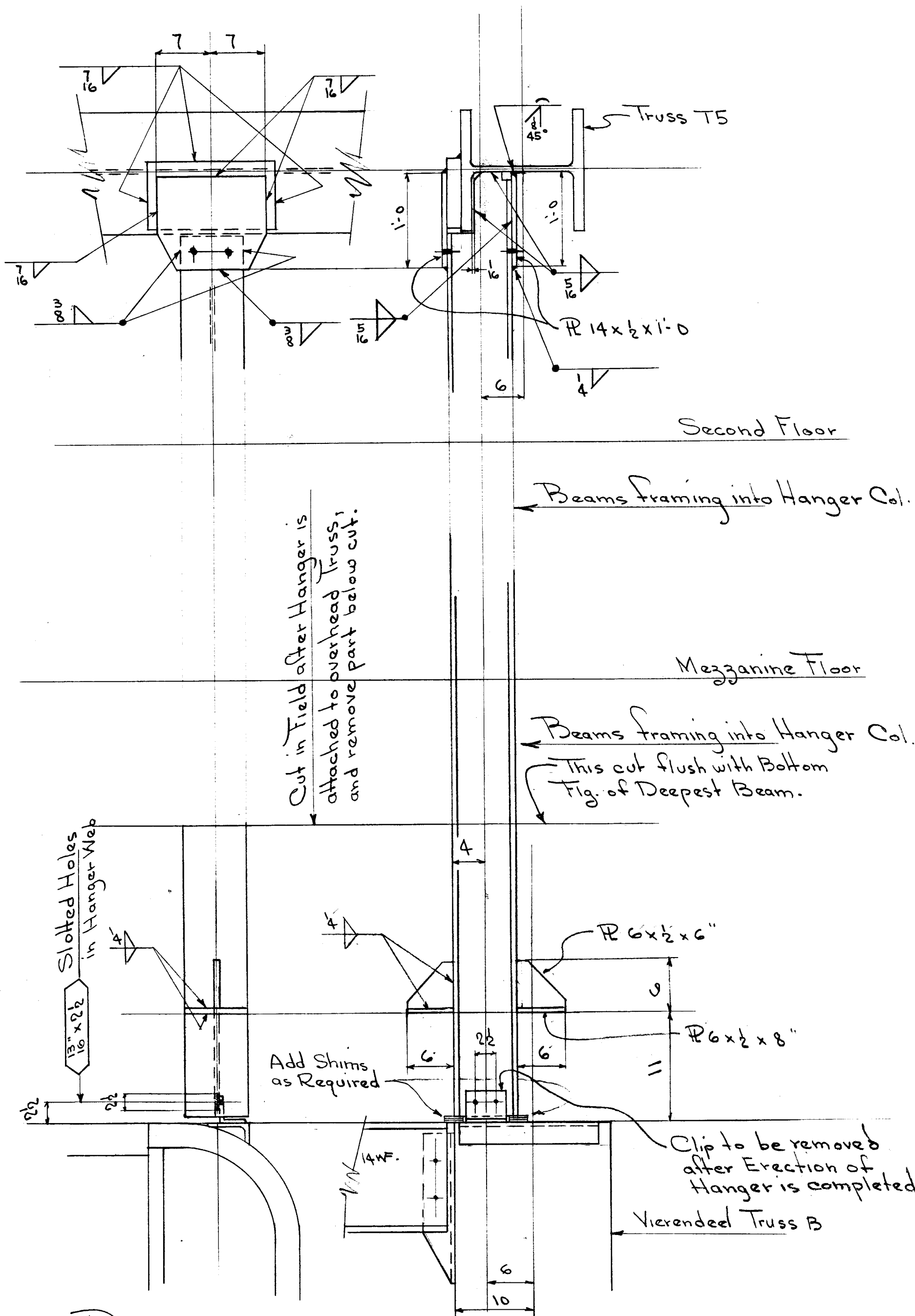
PROPOSED METHOD OF ERECTING HANGER COL. H1
