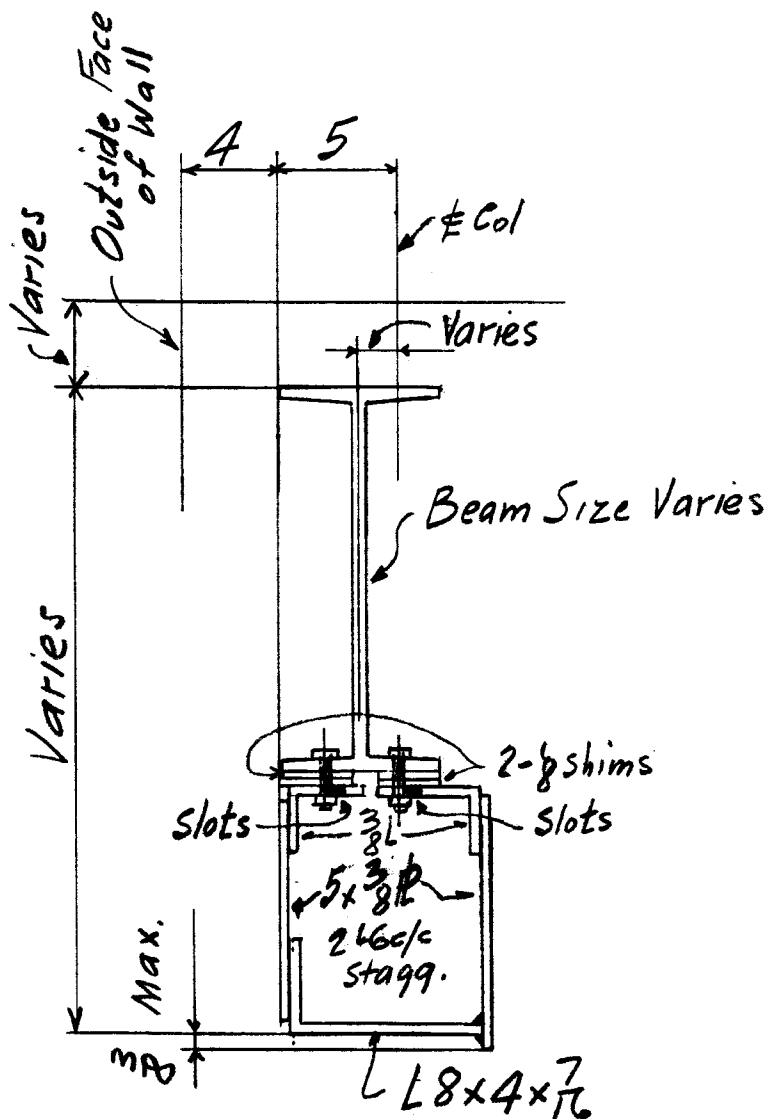
Lintel L1 to Beams
