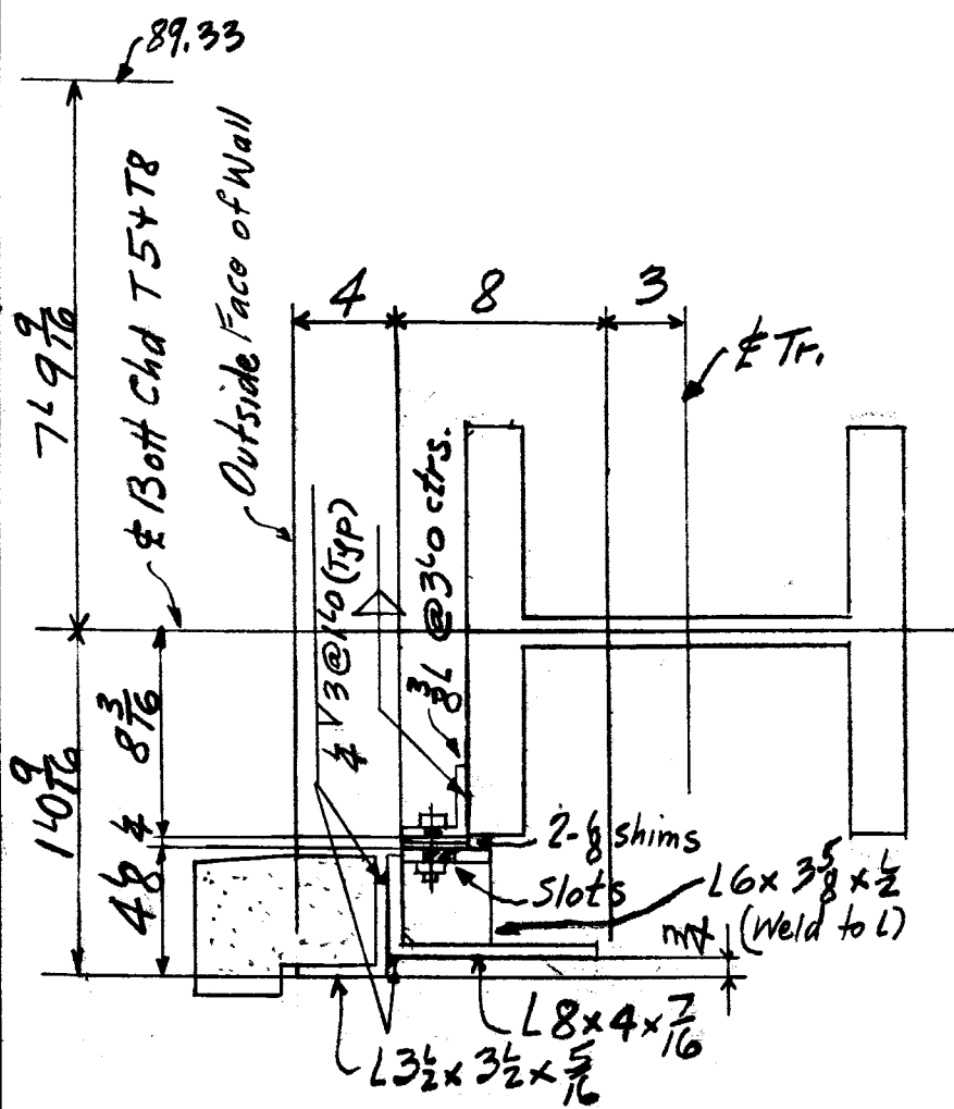
Lintel L2 @ Truss T5+T8
