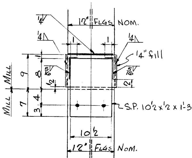
COLUMN SPLICES WITH 1/4" + thk FILLERS OR THICKER
