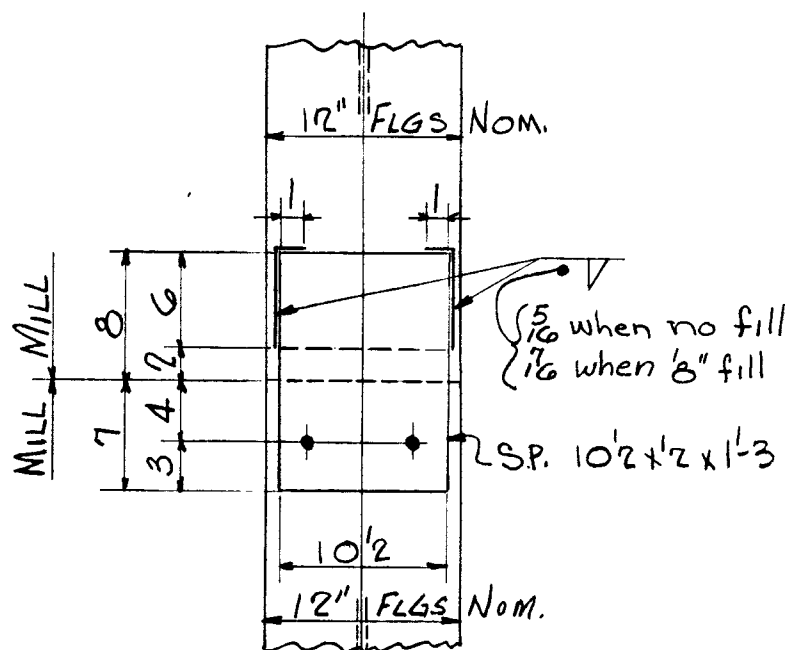
COLUMN SPLICES WITH OR WITHOUT 8" FILLERS
