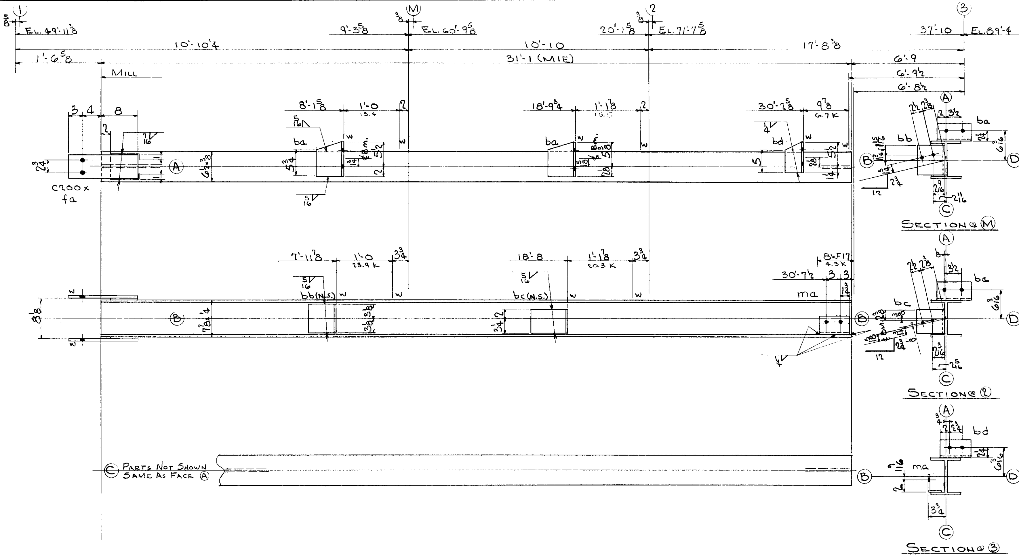
ONE COLUMN - MK. H59 (1-3) FACE (A) SOUTH
