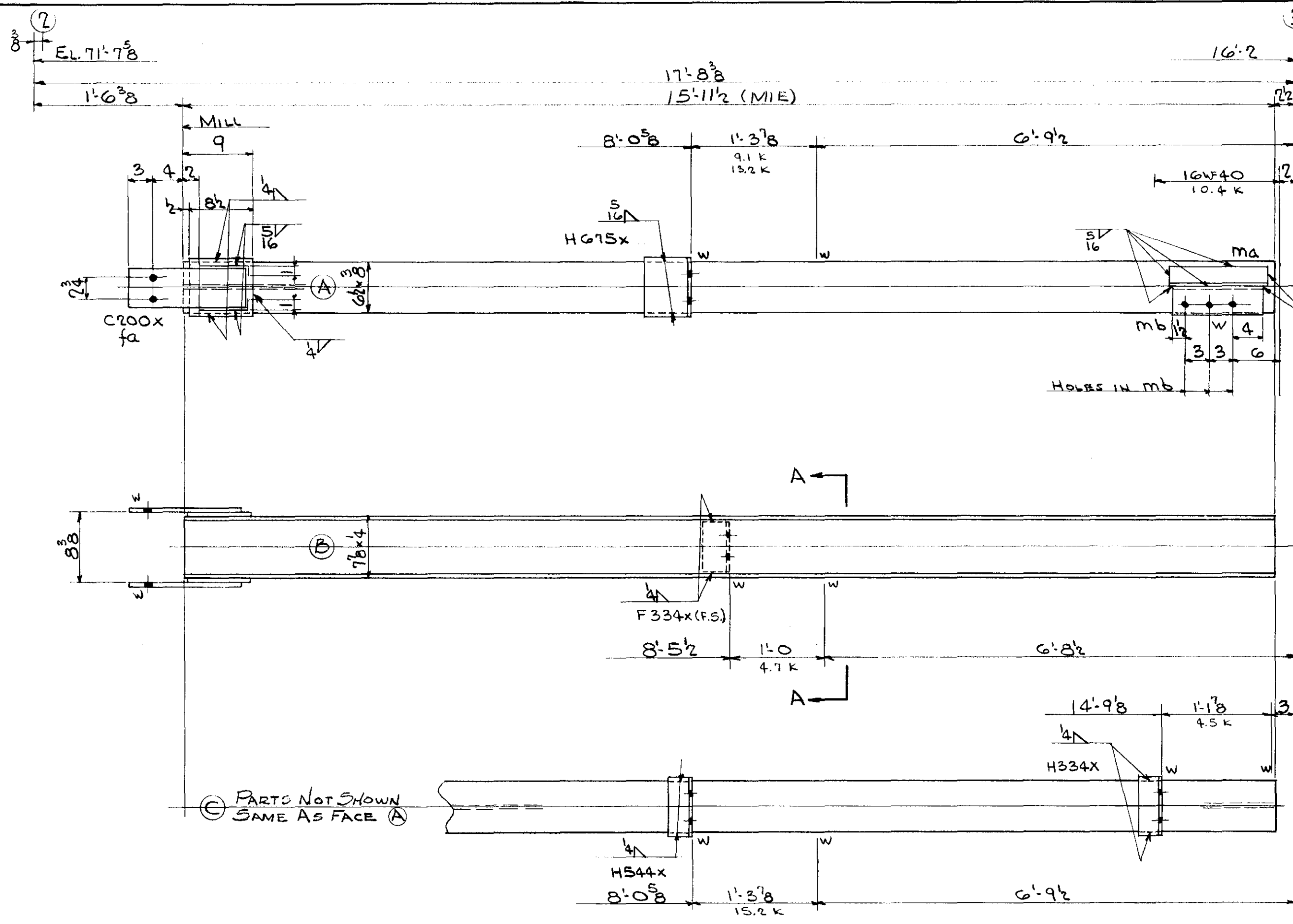
ONE COLUMN - MK. H44 (2-3) FACE (A) SOUTH
