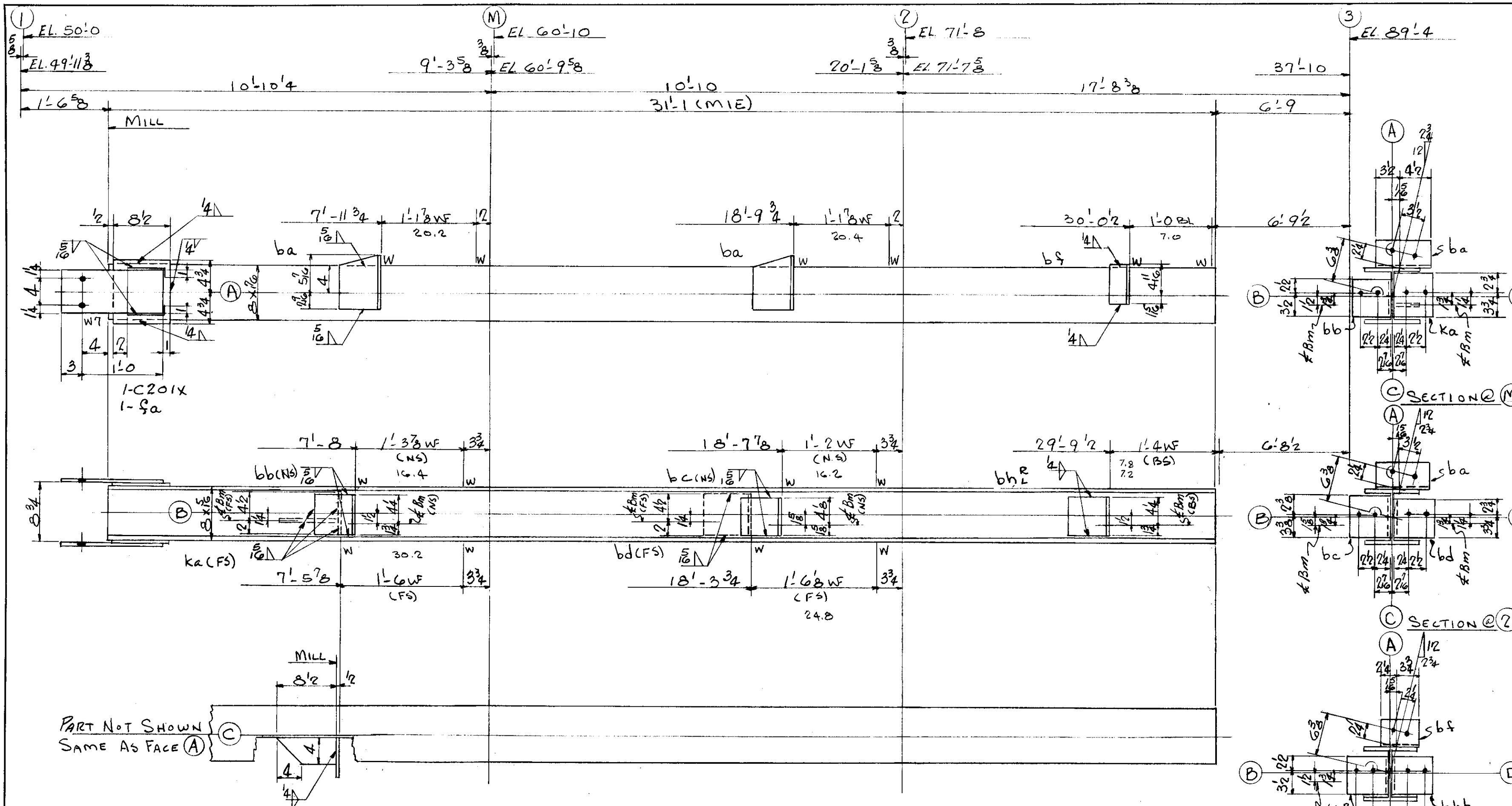
ONE COLUMN MK. H49 (1-3) - FACE (A) SOUTH
