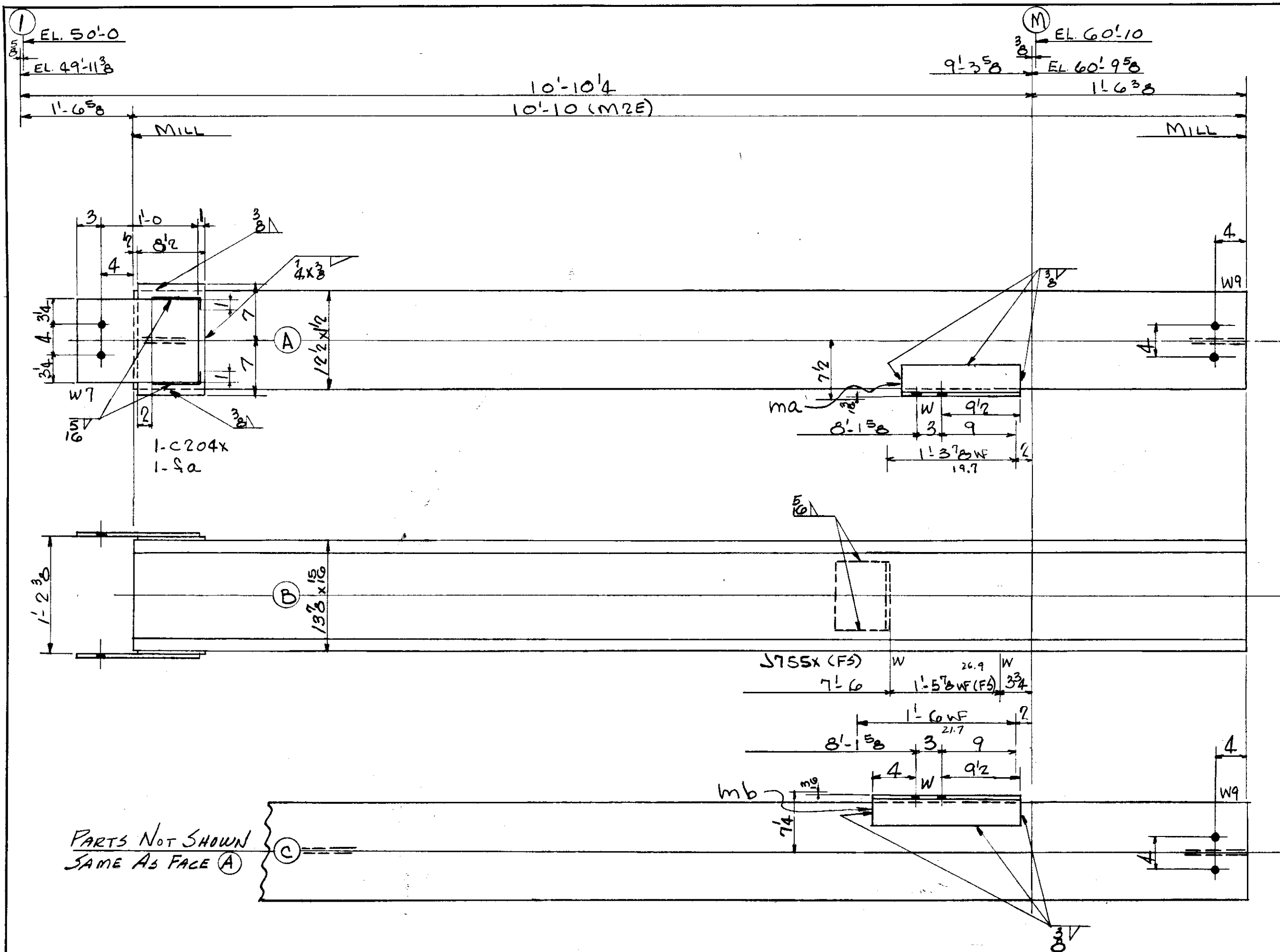
ONE COLUMN MK. C14 (1-m) - FACE (A) SOUTH
