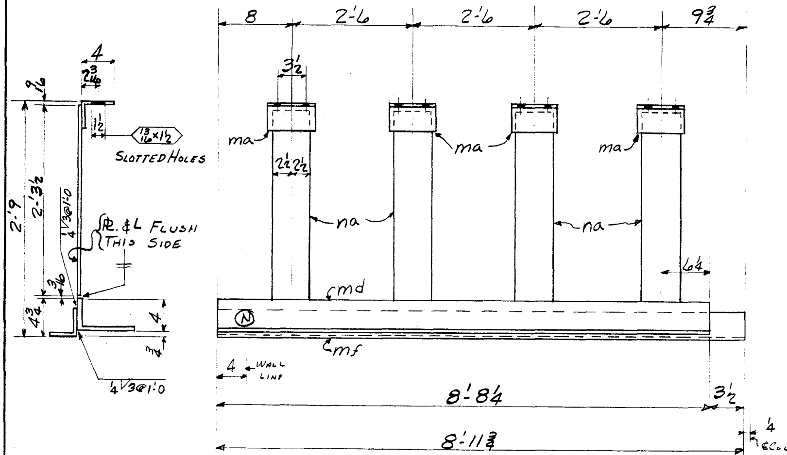
(AS SHOWN) ONE LINTEL MK. CL139 2
