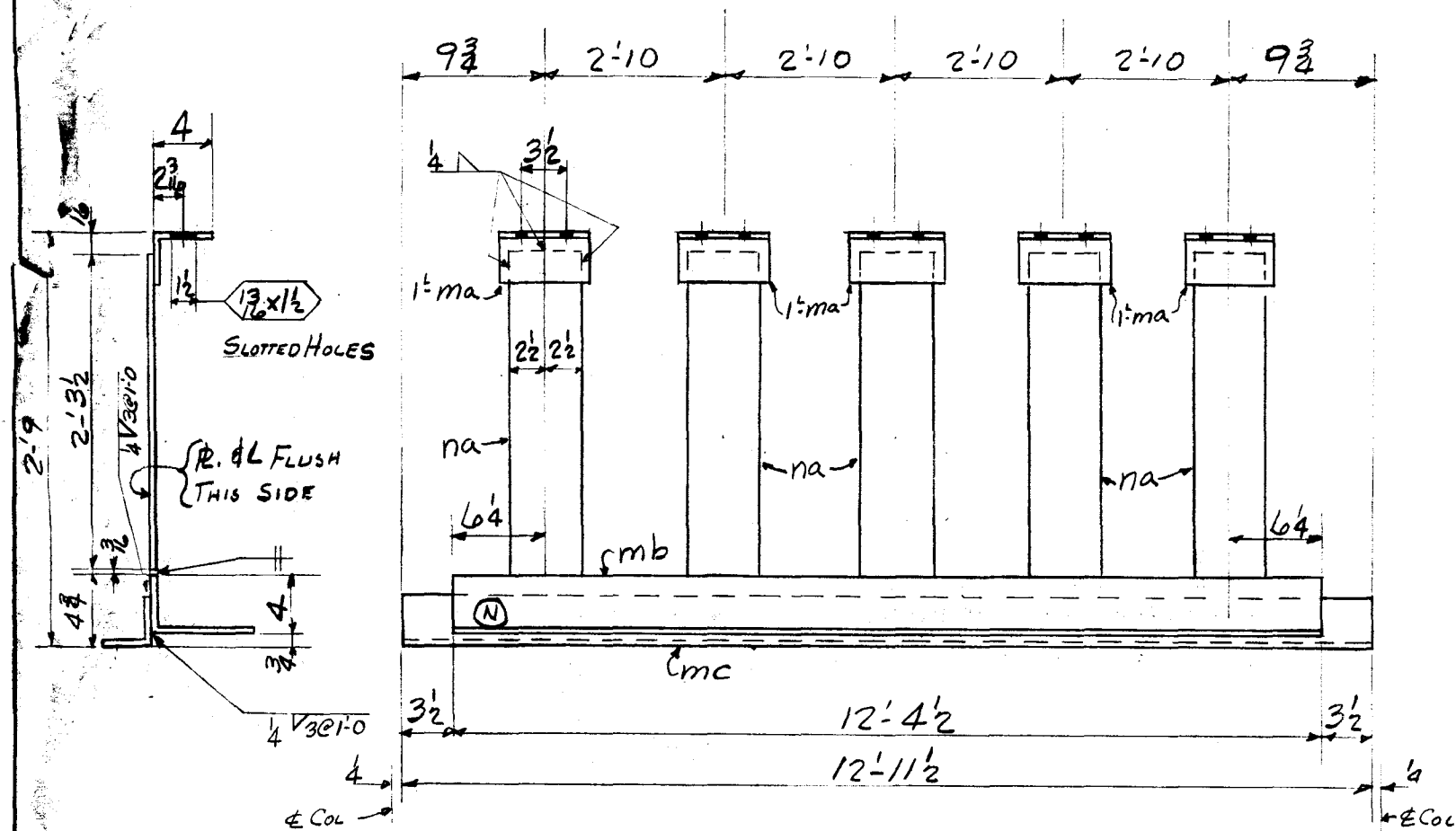
3 LINTELS MK. CL140 3
