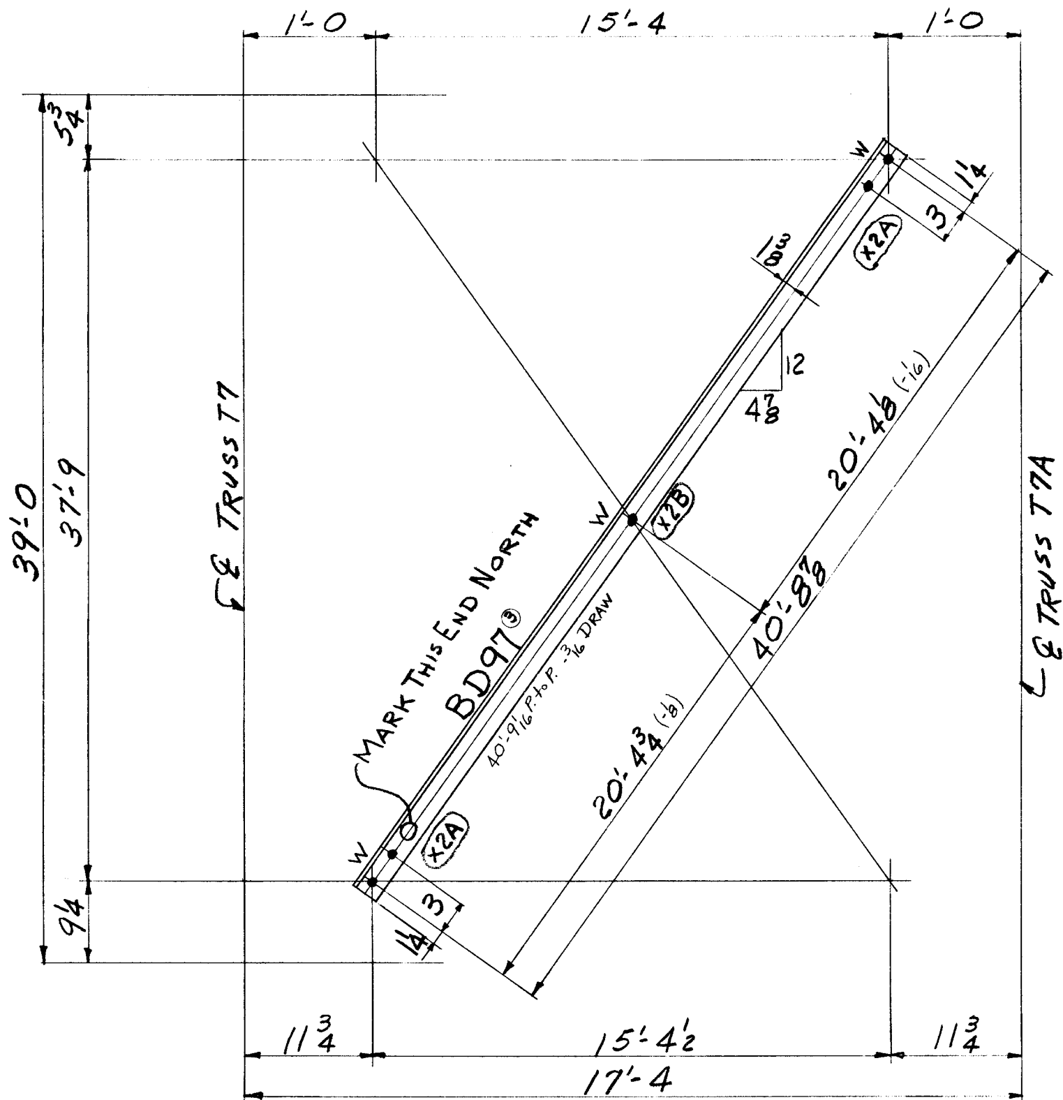
2-DIAGONALS MK. BD97 3
