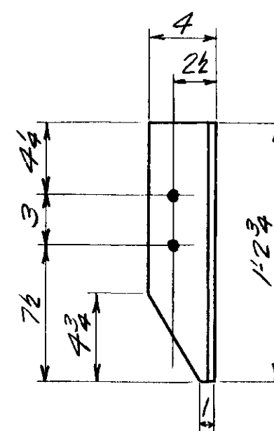
(AS SHOWN) 2-ANGLES MK. A1-22; A2-22 (OPP. HAND) 2-ANGLES MK. A1-33; A2-33 } (ONE EA.)
