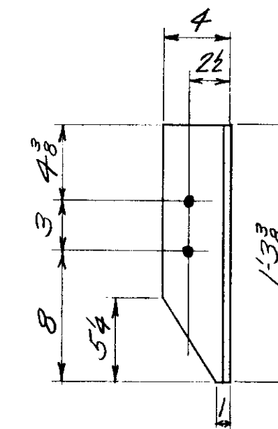
(AS SHOWN) 4- ANGLES MK. A1-23; A2-23 (OPP. HAND) 4- ANGLES MK. A1-34; A2-34 } (2 EA.)
