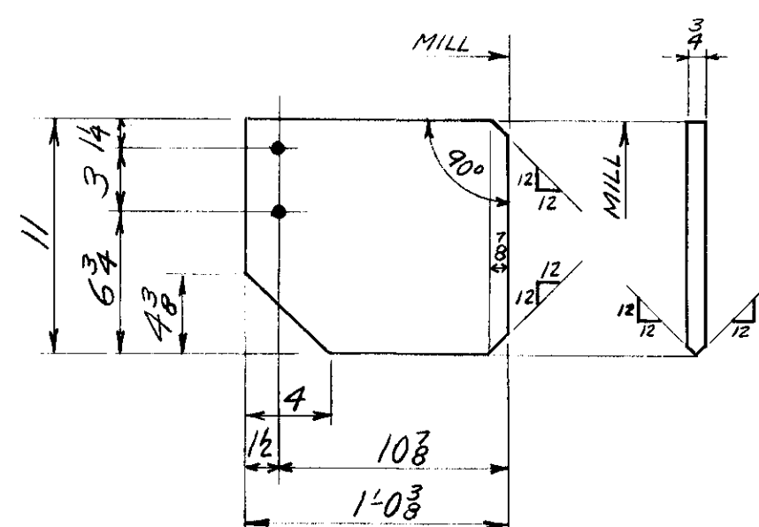
6- PLATES MK. A1-12; A2-12 (3EA.)
