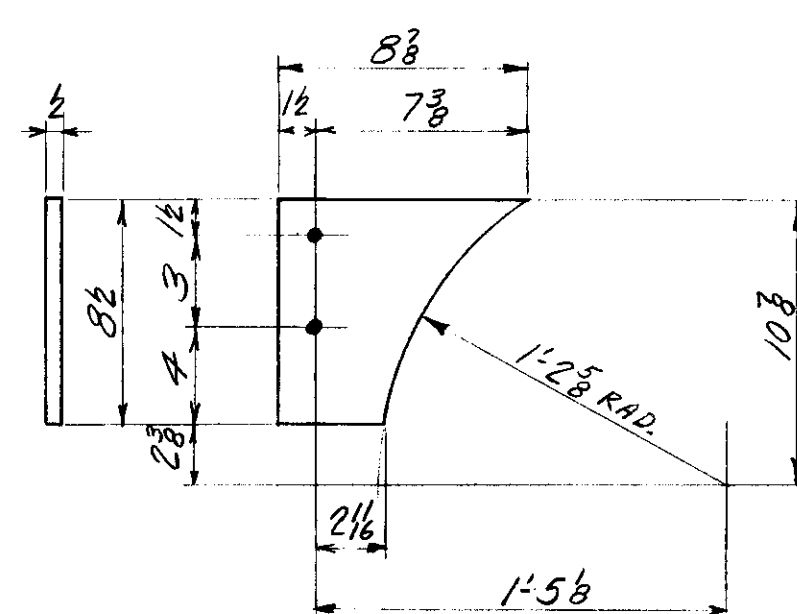
2-PLATES MK A1-16; A2-16 (ONE EA.)
