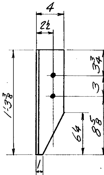
(AS SHOWN) 2-ANGLES MK. A1-21 (OPP. HAND) 2-ANGLES MK. A2-32
