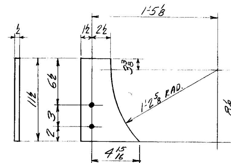
2 - PLATES MK. A1-17; A2-17 (ONE EA.)
