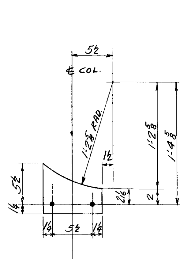
2- PLATES MK. A1-24; A2-24 (ONE EA.)
