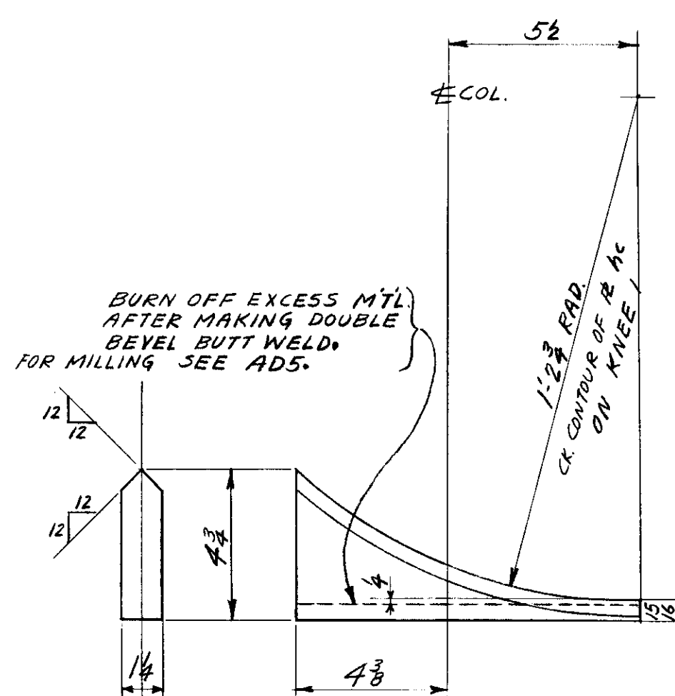
2-PLATES MK. A1-25; A2-25 (ONE EA.)
