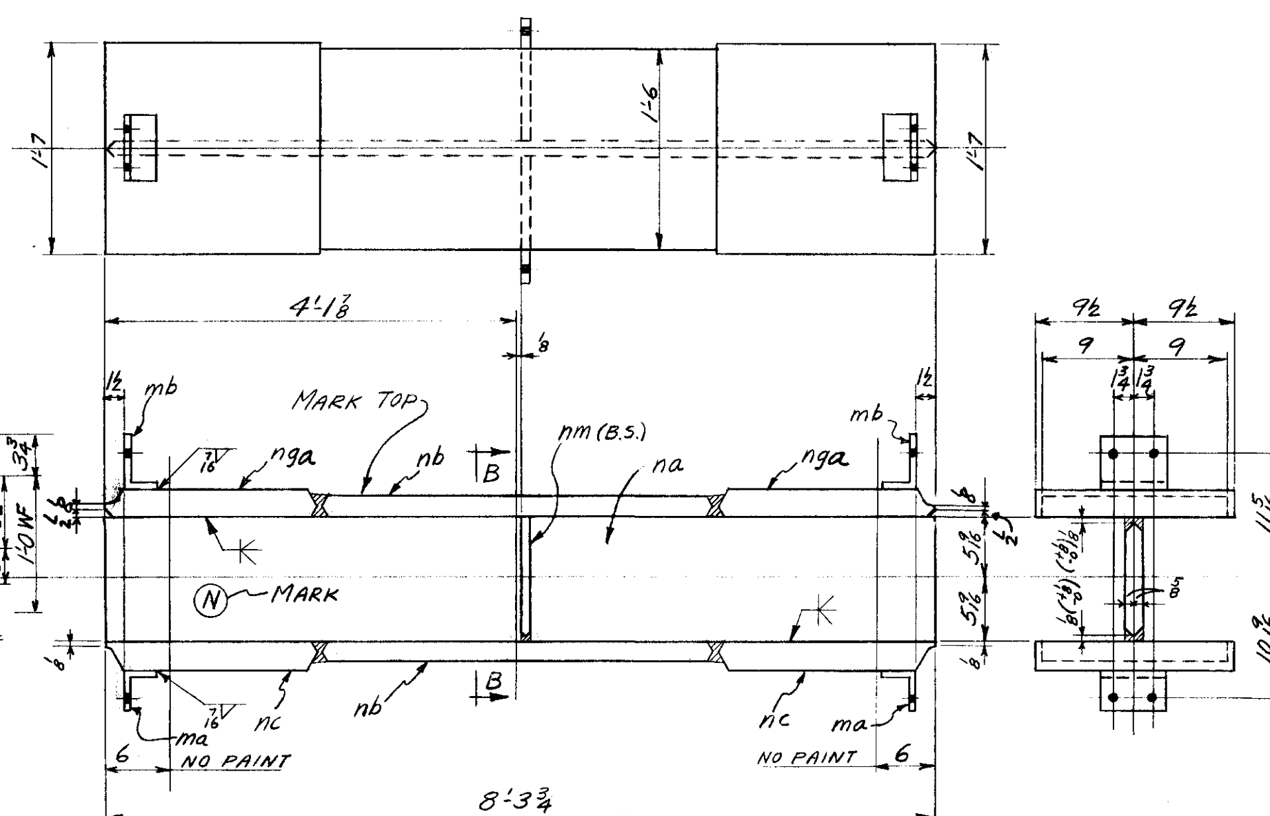
ONE-CHORD MK. DA-30
