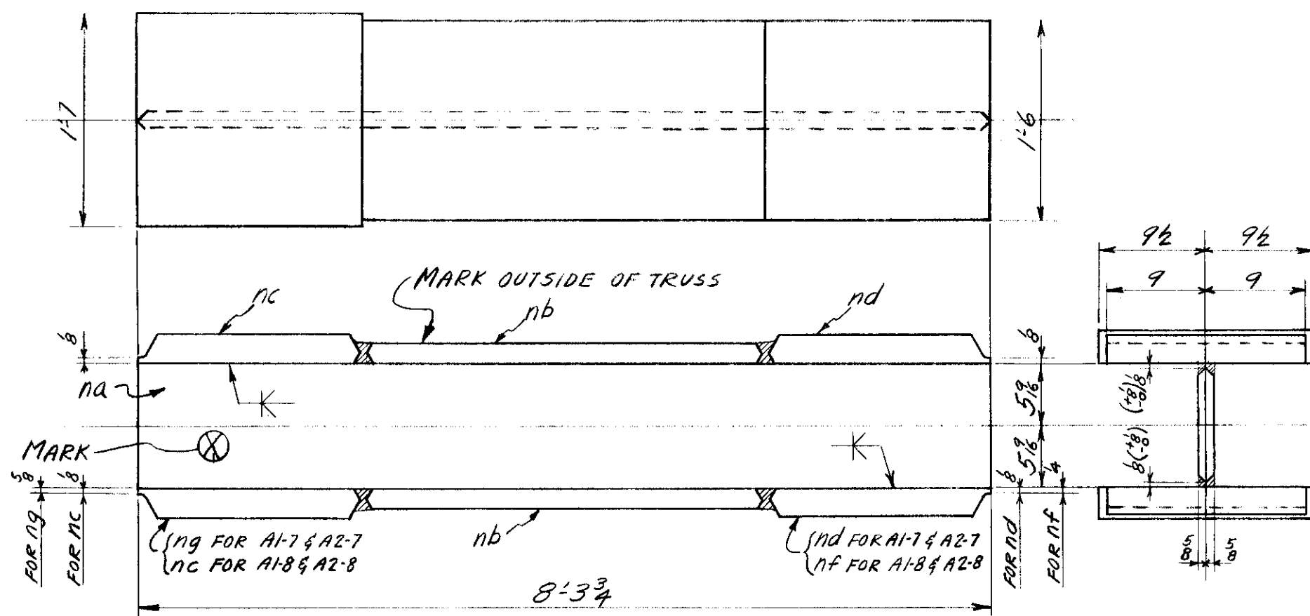
8-CHORDS MK. A1-7; A2-7; A1-8; A2-8 (2EA.)
