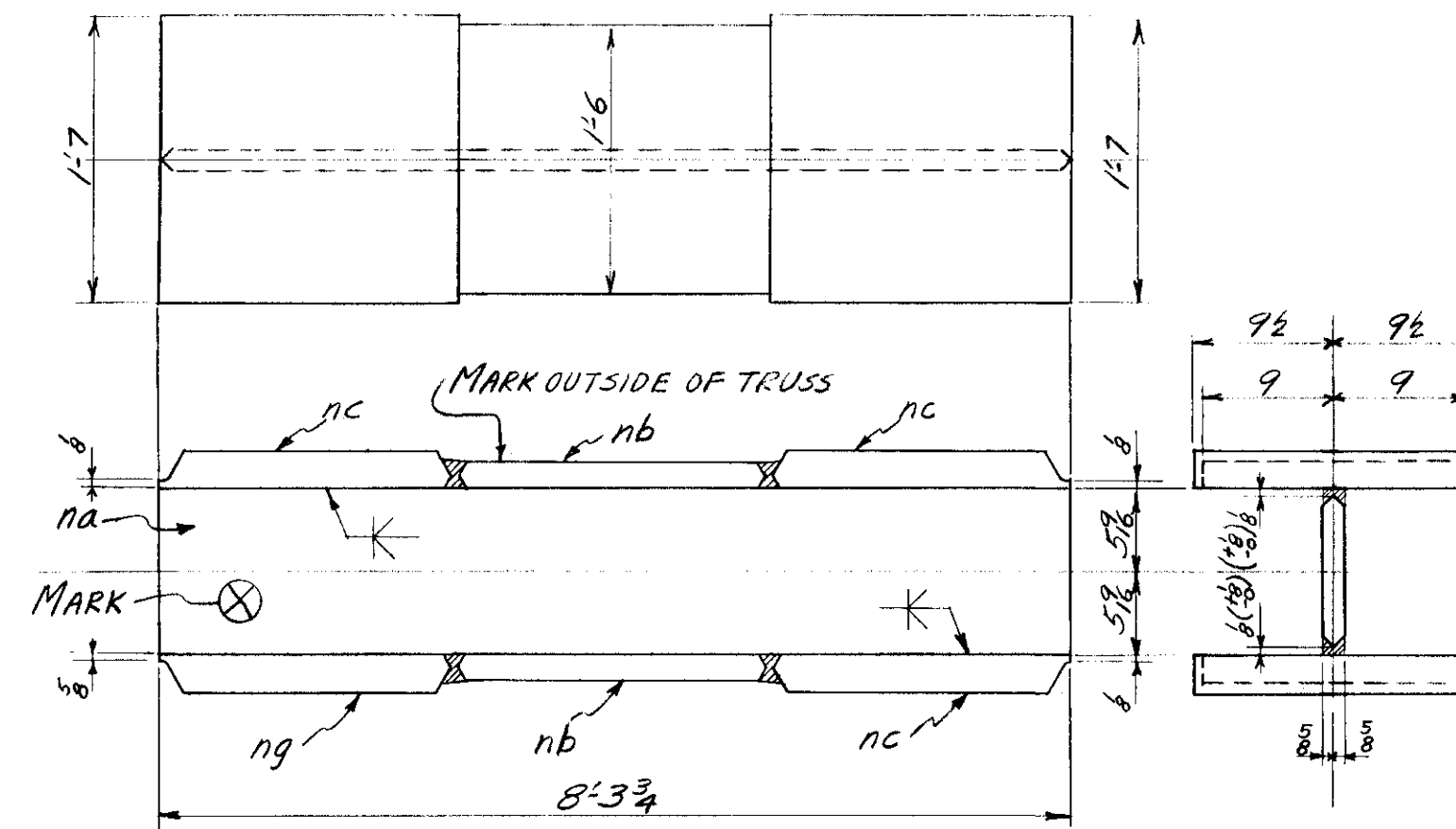
4-CHORDS MK. A1-9; A2-9 (2EA.)
