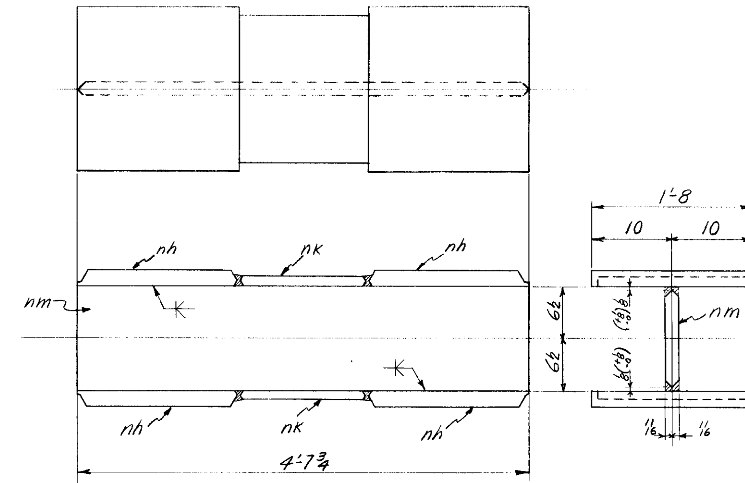
4 - VERTICALS MK. A1-6; A2-6; (2 EA)
