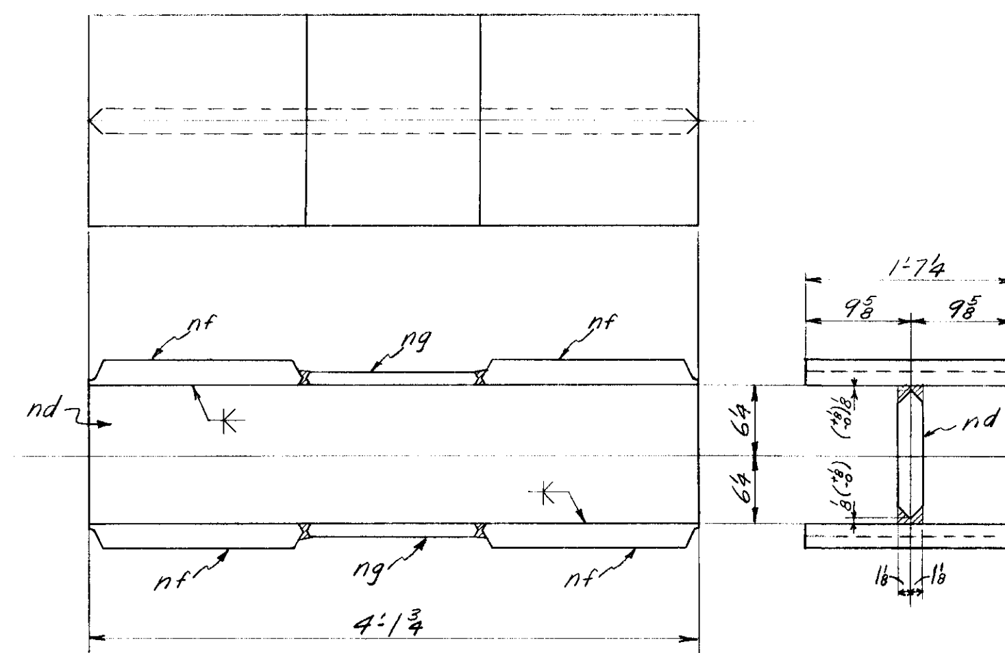
2 - VERTICALS MK. A1-5; A2-5; (ONE EA)
