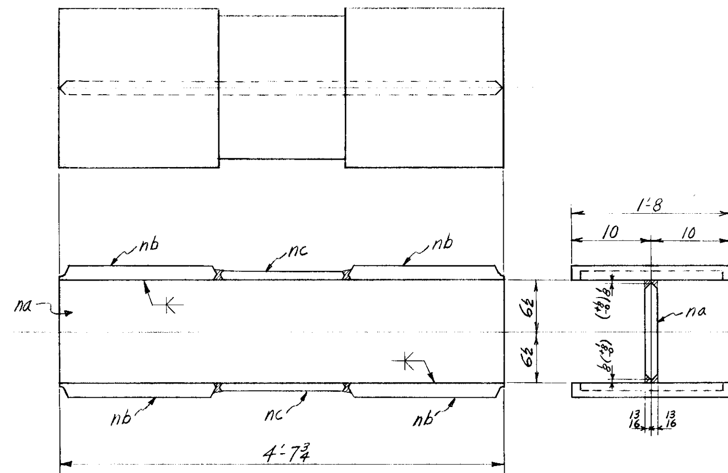
2 - VERTICALS MK. A1-4; A2-4; (ONE EA)
