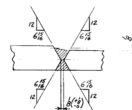
TYPICAL WELDING FOR ALL FLANGE JOINTS
