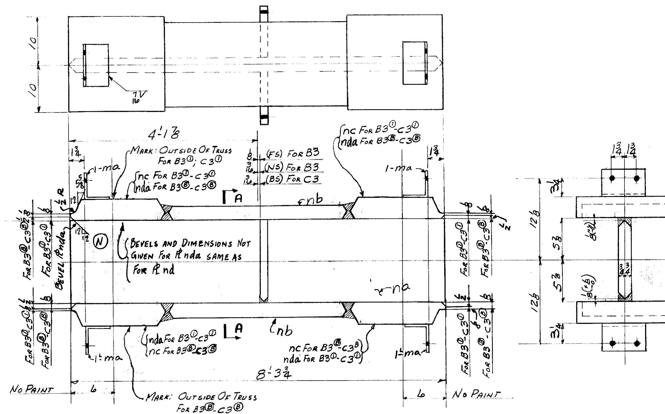
4 CHORDS M_kCB3^{(B)} - CB3^{(1)} - CC3^{(B)} - CC3^{(1)} (ONE EACH)
