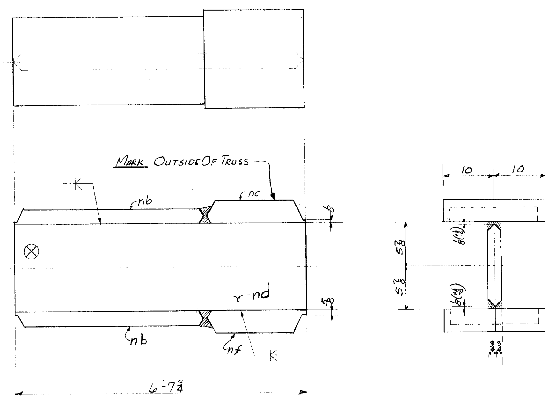
8 CHORDS Mk. B1-11; C1-11; B2-11; C2-11 (2 EACH)
