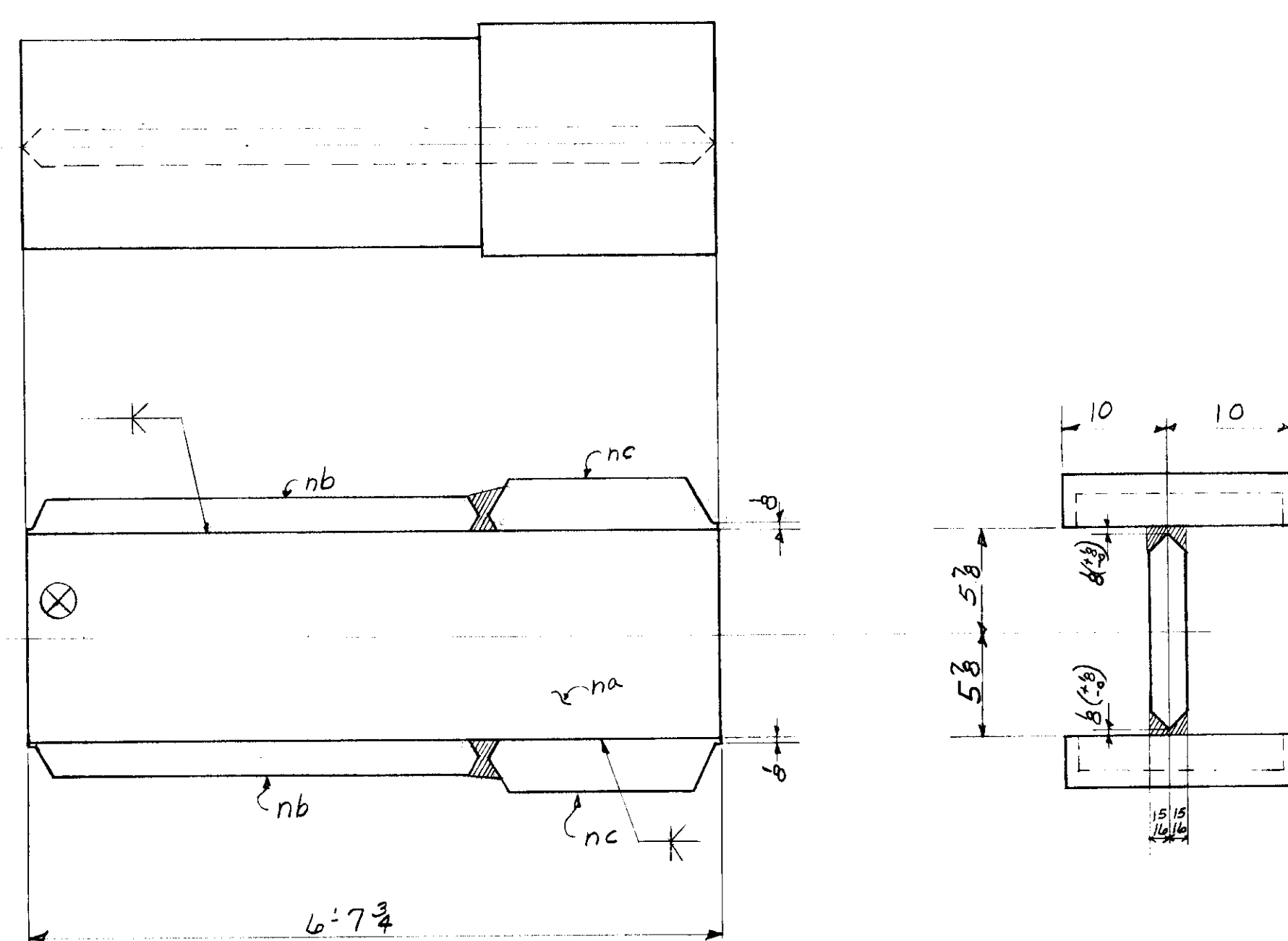
8 CHORDS Mk. B1-10; C1-10; B2-10; C2-10 (2 EACH)
