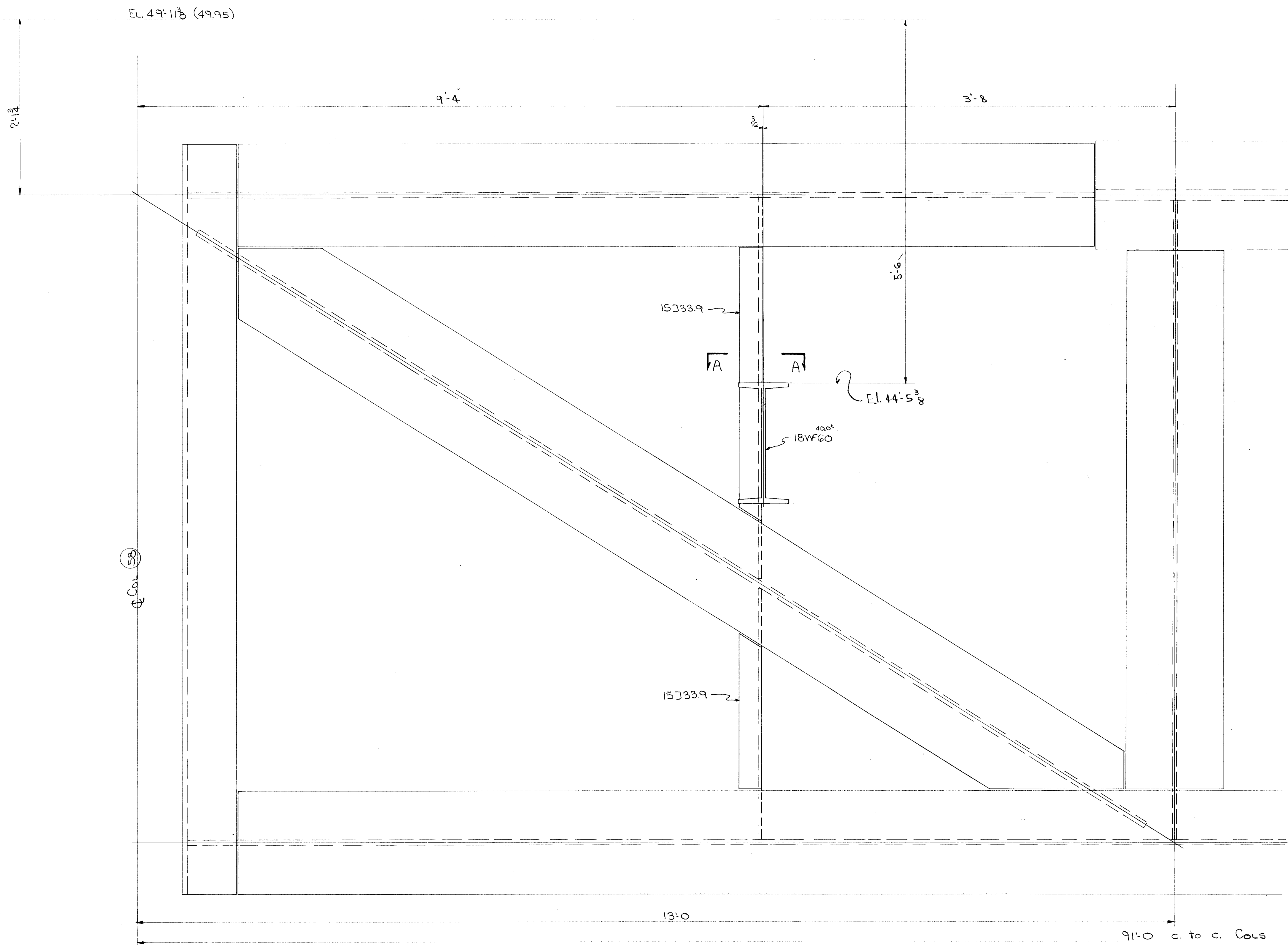
SOUTH END TRUSS T4
