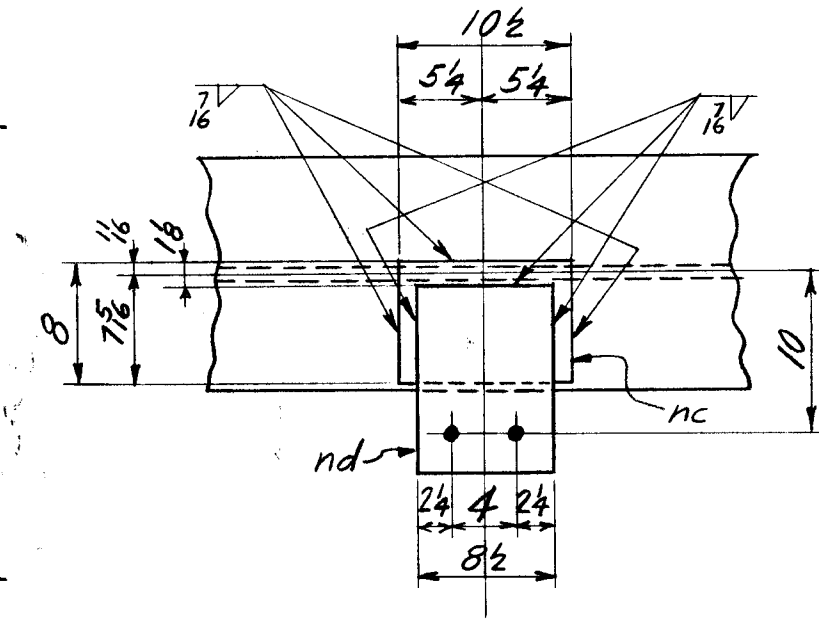
SECTION E-E
