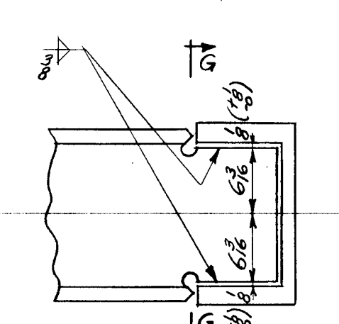
TYPICAL WEB CONN. FOR DIAGONAL MEMBER WF
