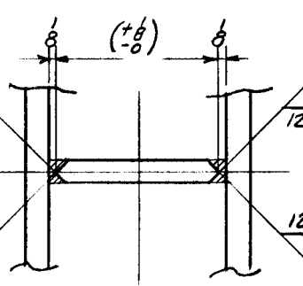
SECTION G-G
